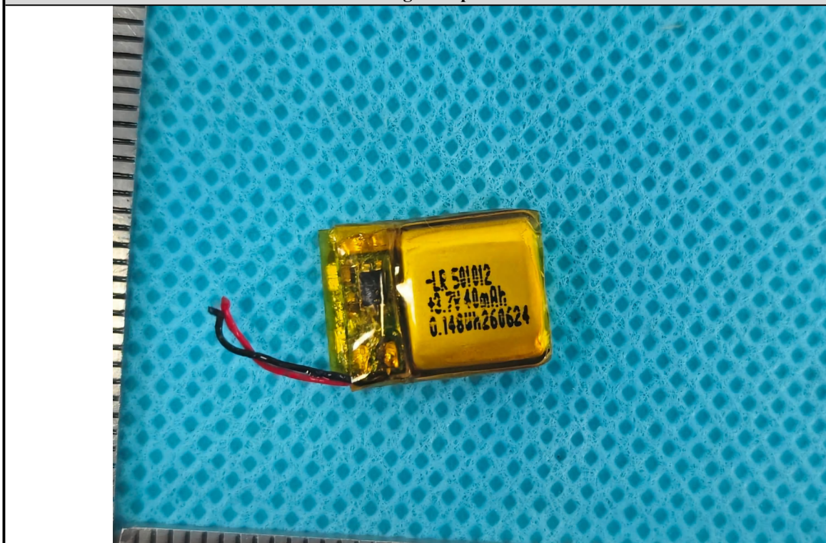
Right earphone Photo
