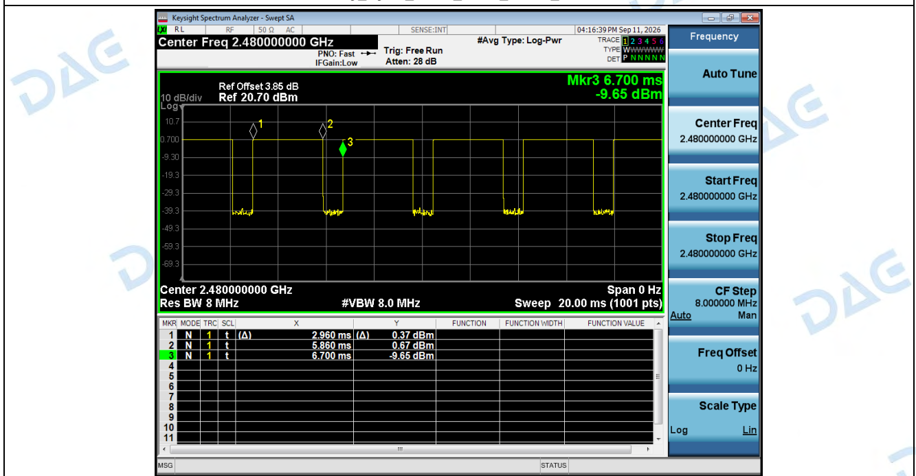
Duty_Cycle_NVNT_ANT1_1-DH5_2480
