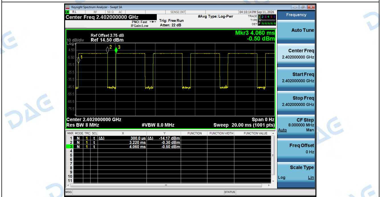
Duty_Cycle_NVNT_ANT1_1-DH5_2402
