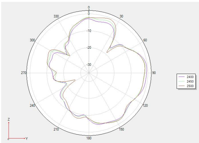
Phi 90 2Dgraph
