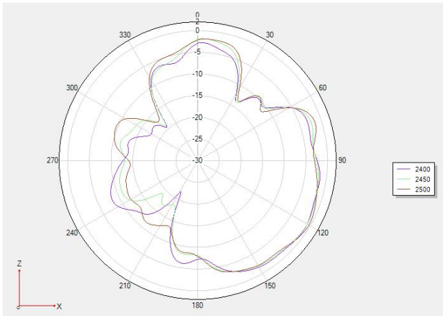
Phi 0 2Dgraph
