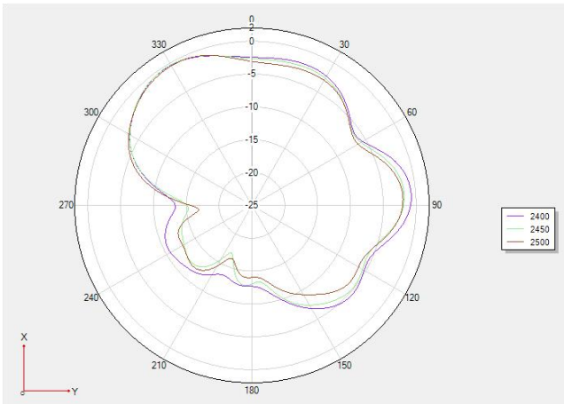
Theta 90 2Dgraph
