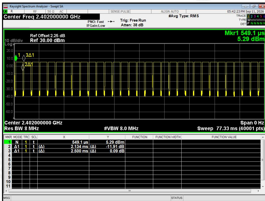
Test Chart - 2402MHz
