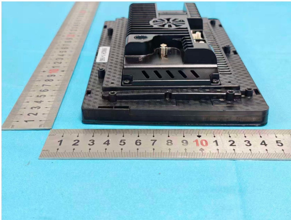
Photo 9 External photos of EUT
