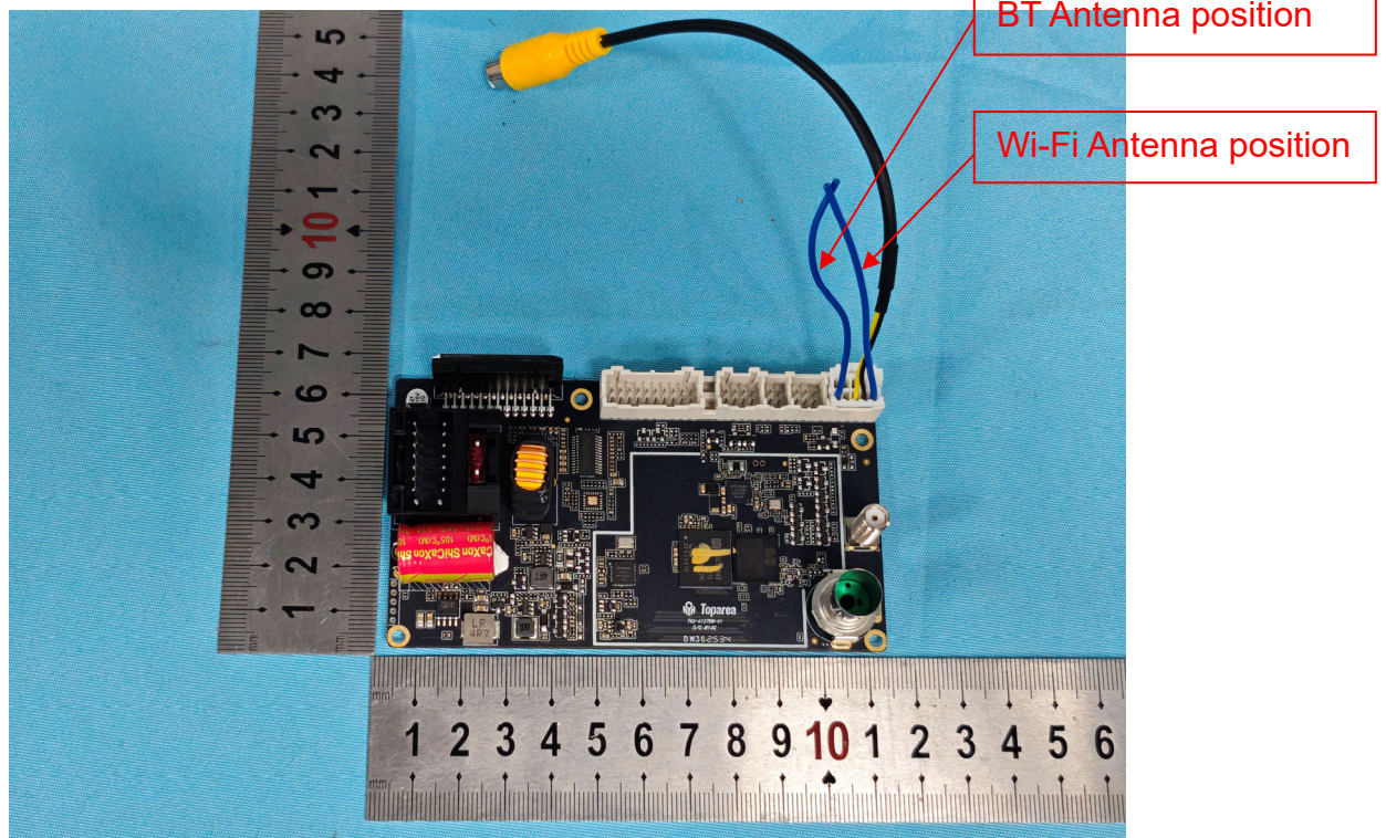
Photo 2 Internal photos of EUT
