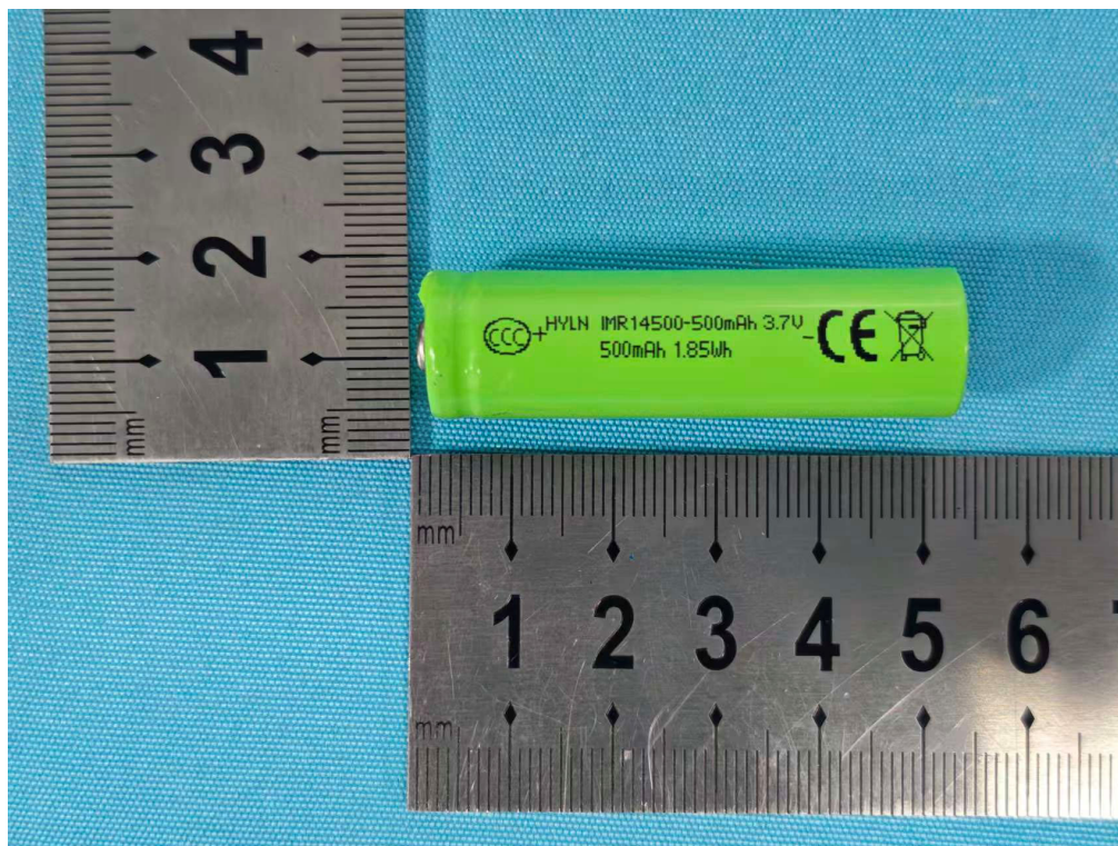
Photo 7 Internal photos of EUT
