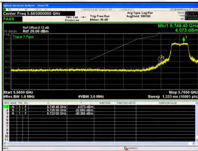
802.11ac(VHT40)-5755
