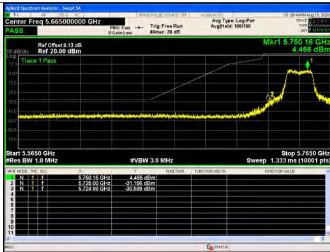
802.11ac(VHT20)-5745
