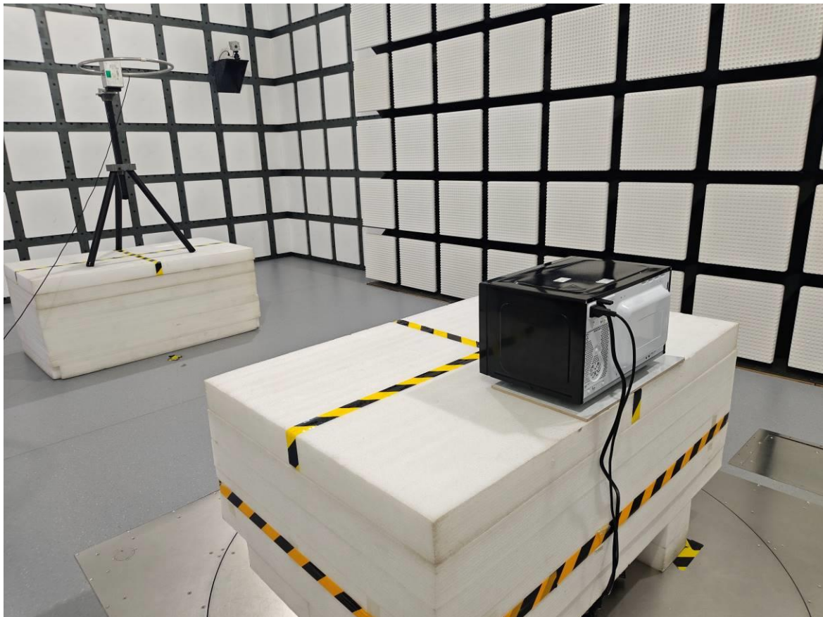
Radiated Emission 9 kHz-30 MHz Ground-parallel Rear View
