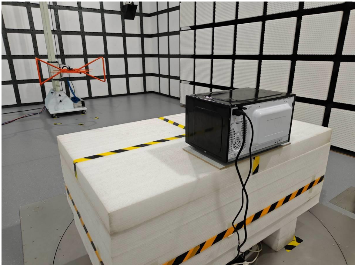
Radiated Emission 30 MHz-1 GHz Rear View
