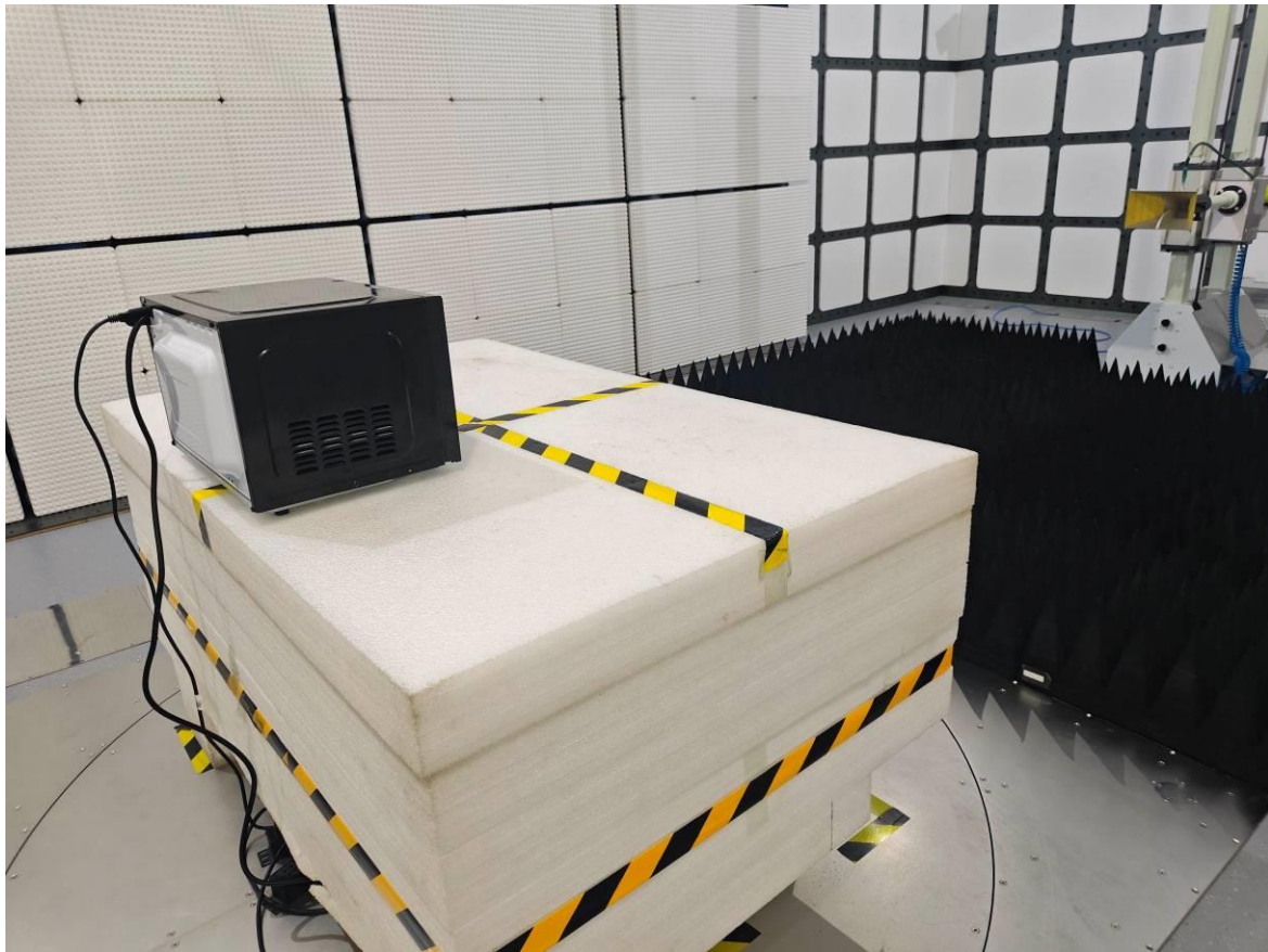
Radiated Emission Above 1GHz Rear View
