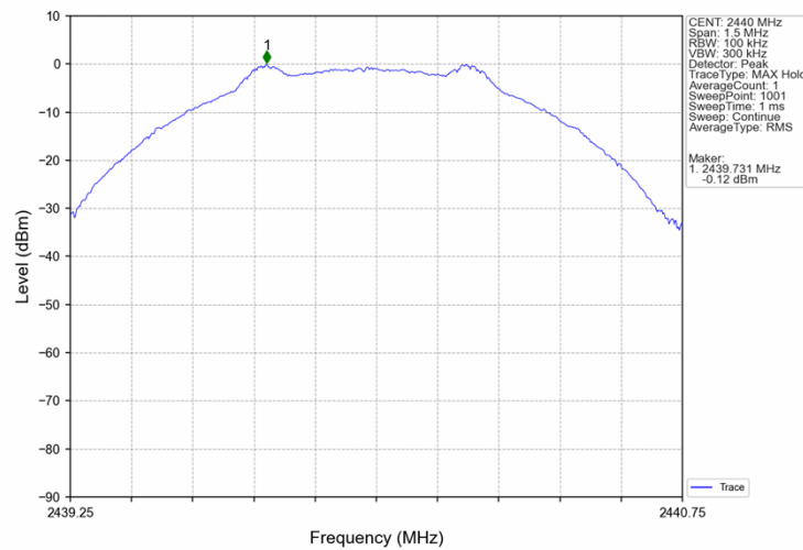
1M_MCH_2440MHz_Ant1_NTNV
