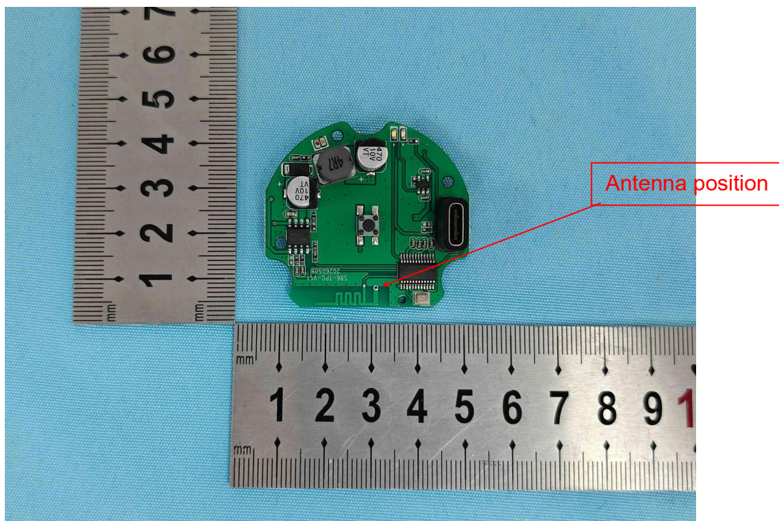
Photo 2 Internal photos of EUT
