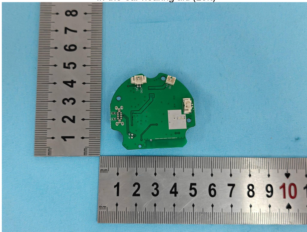
Photo 3 Internal photos of EUT In-the-ear hearing aid (Left)
