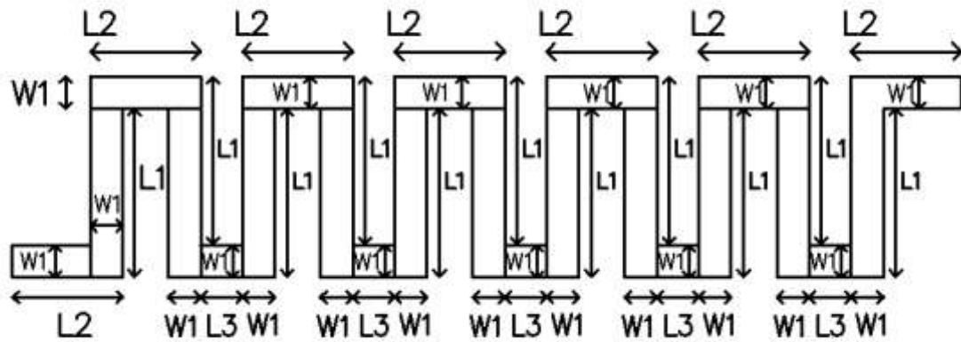
Figure 3:Antenna Dimensions
