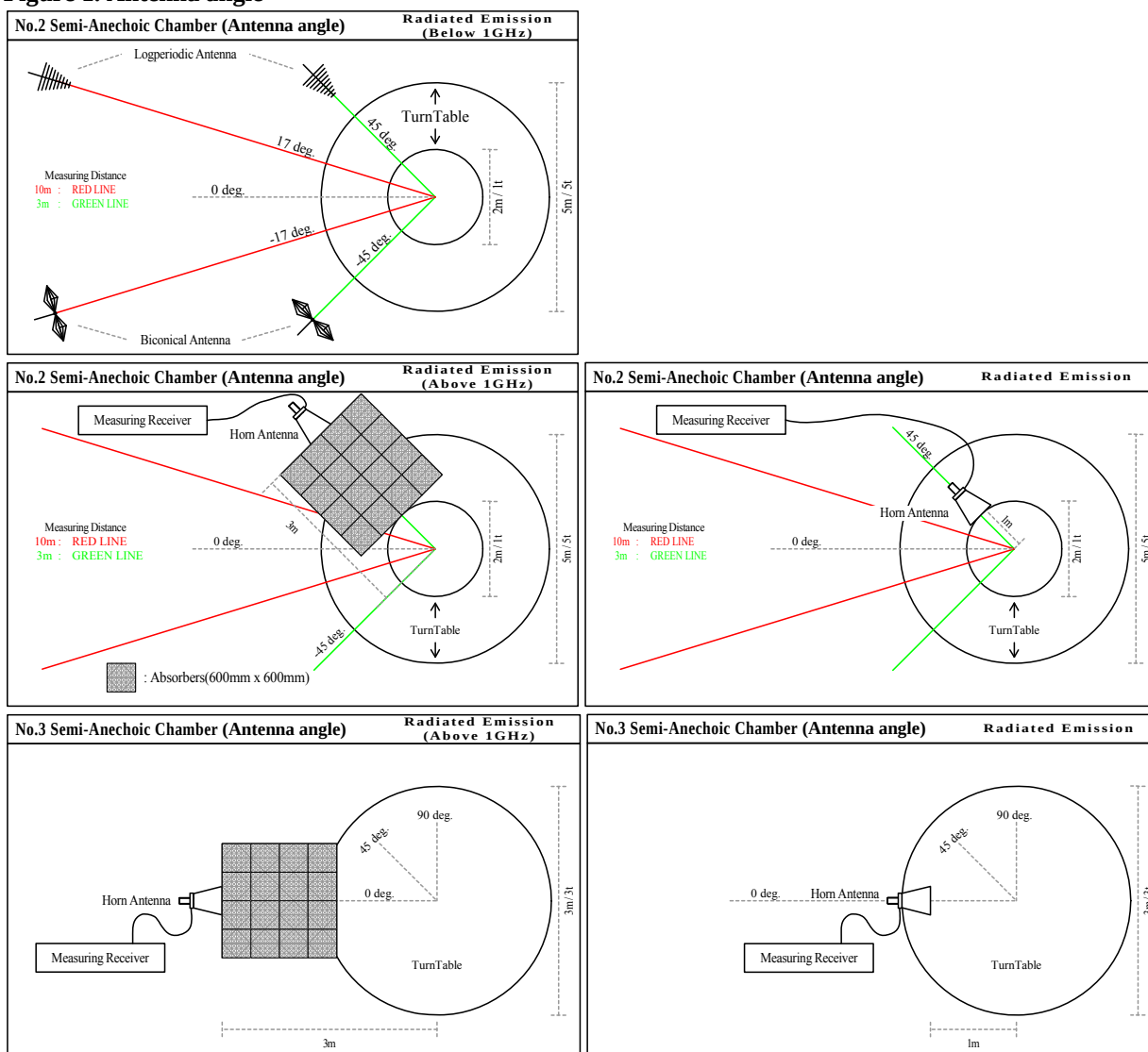
Figure 1. Antenna angle
