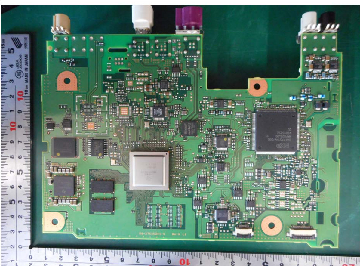
Main PCB Bottom view
