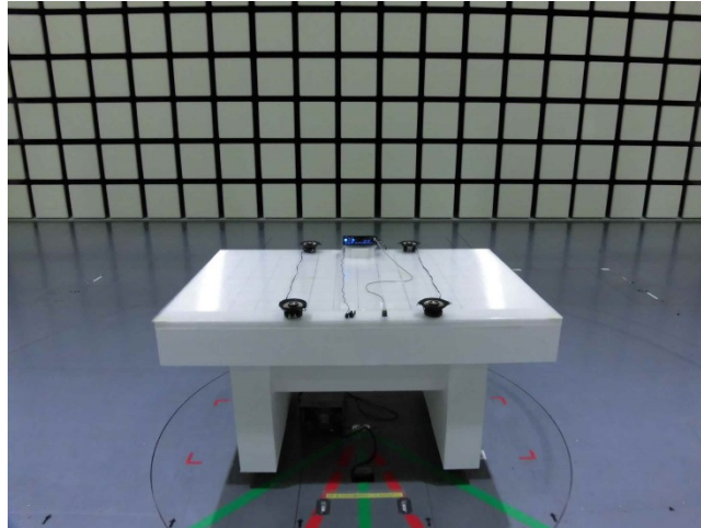
Radiated Spurious Emission Front
