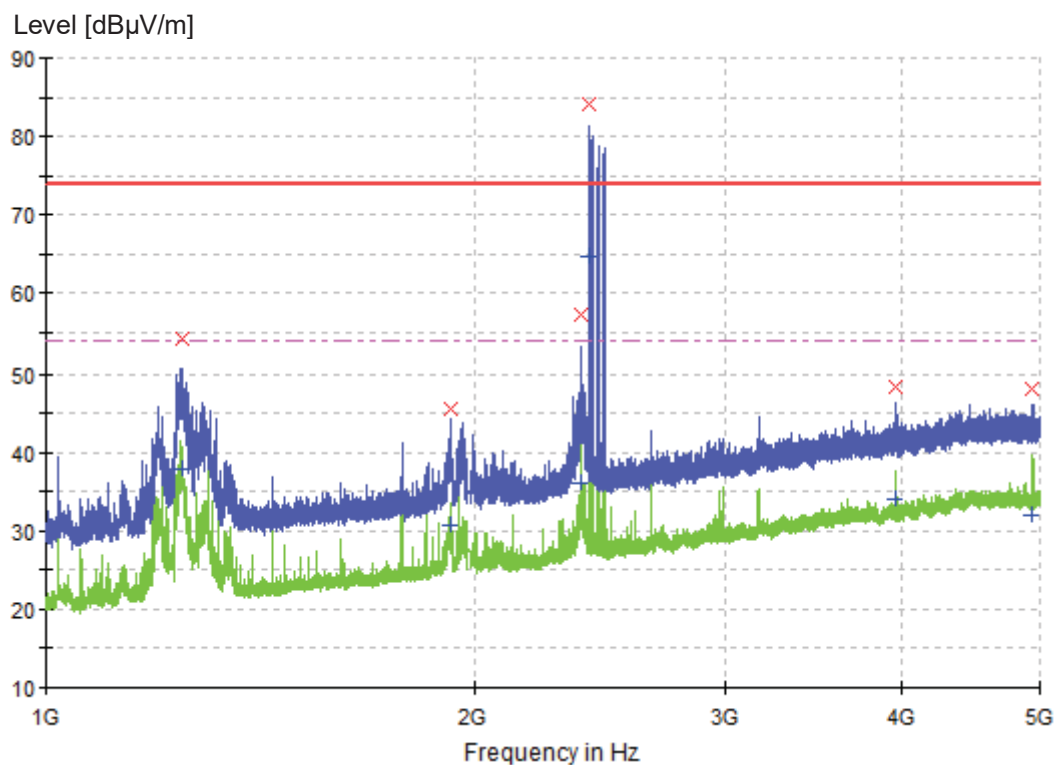
Figure 6: Spectral Diagrams and measurement results, 1 GHz-5 GHz, vertical polarization for mode 1
