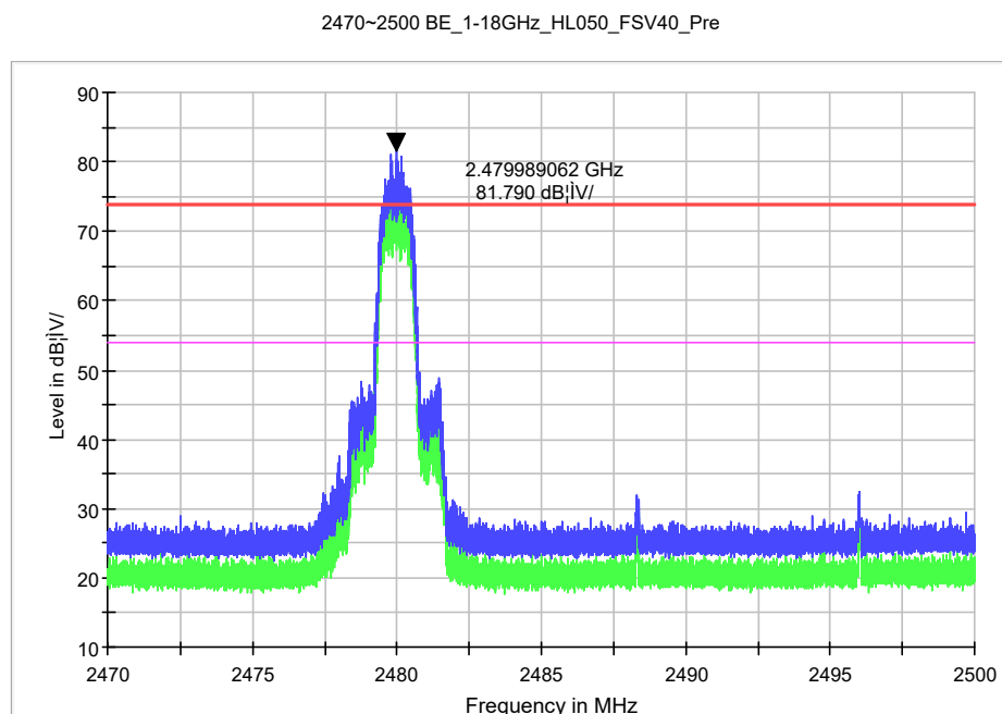
Figure 80: Radiated Band-Edge, TM9, H
