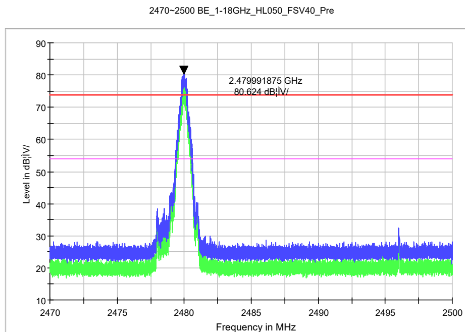
Figure 72: Radiated Band-Edge, TM3, H
