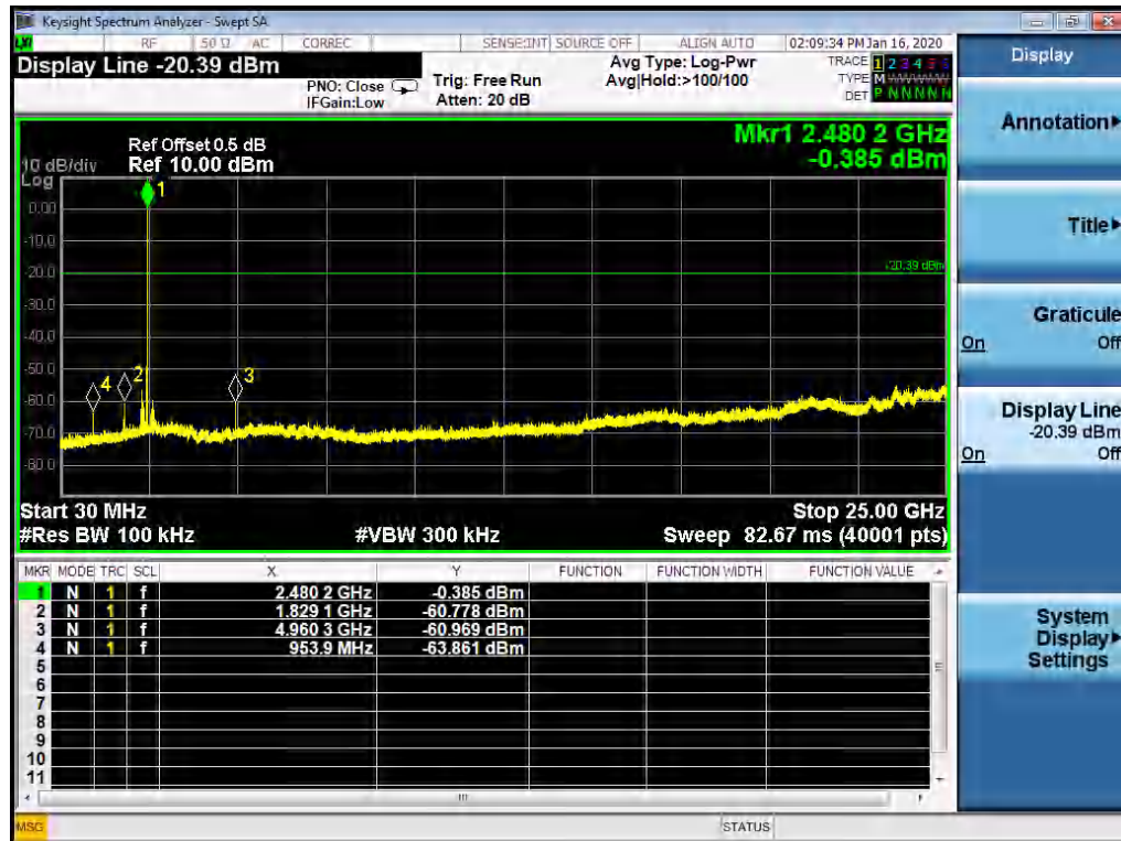
Figure 69: Conducted Spurious Emission, TM9
