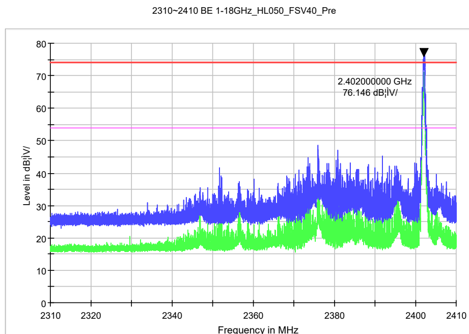
Figure 70: Radiated Band-Edge, TM1, H
