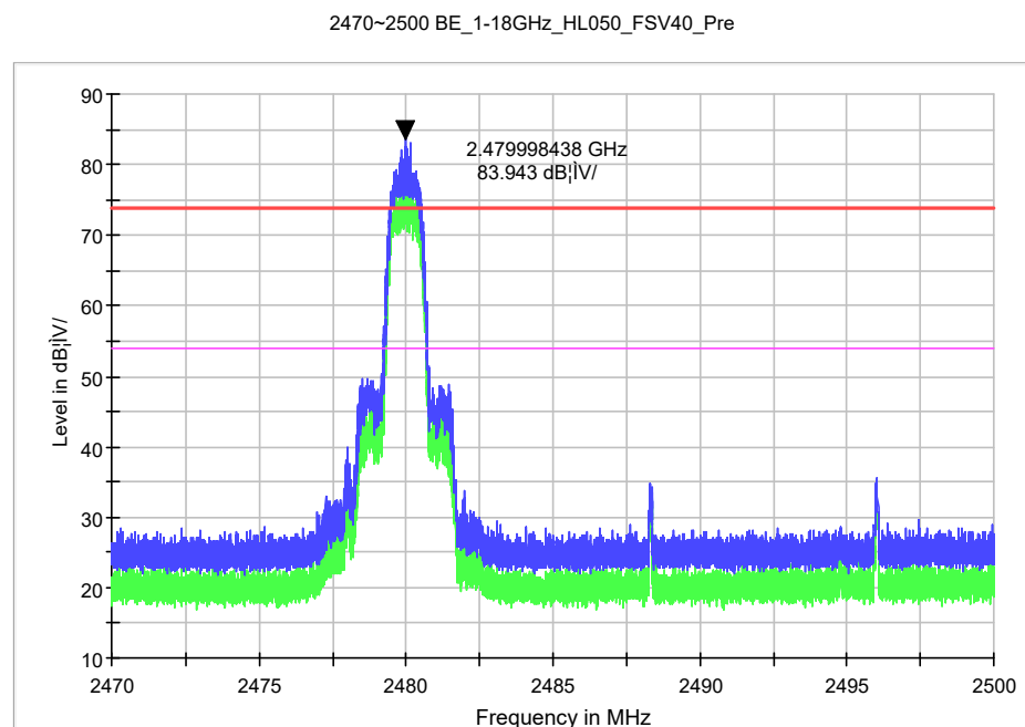
Figure 77: Radiated Band-Edge, TM6, V
