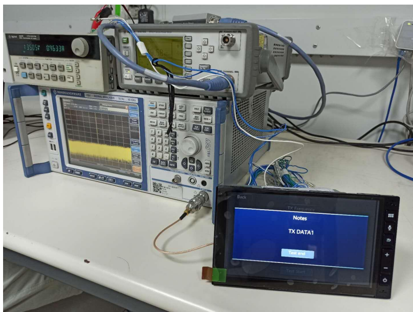
RF Conducted Test setup (BT)
