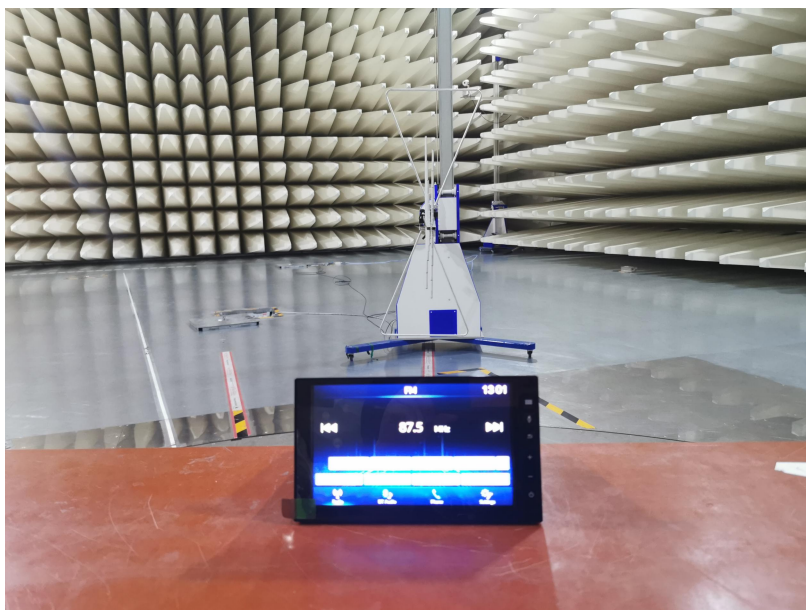
Radiated Emissions Test Setup(below 1GHz)
