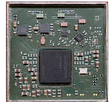
Wifi/BT Module without cover(TOP)
