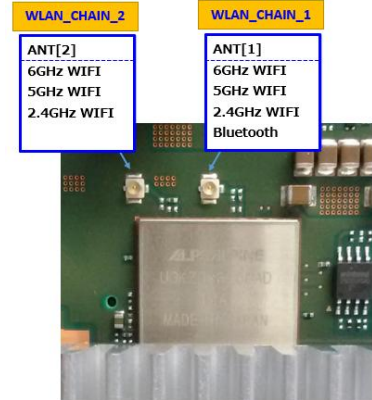
Wifi/BT Module with cover(TOP)
