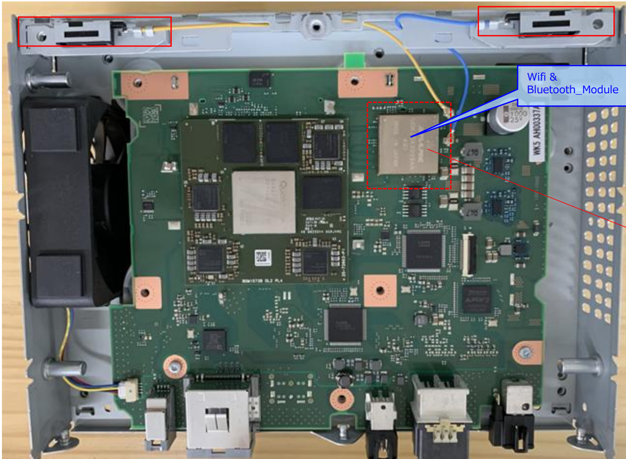
Wifi/BT Module with cover(TOP)
