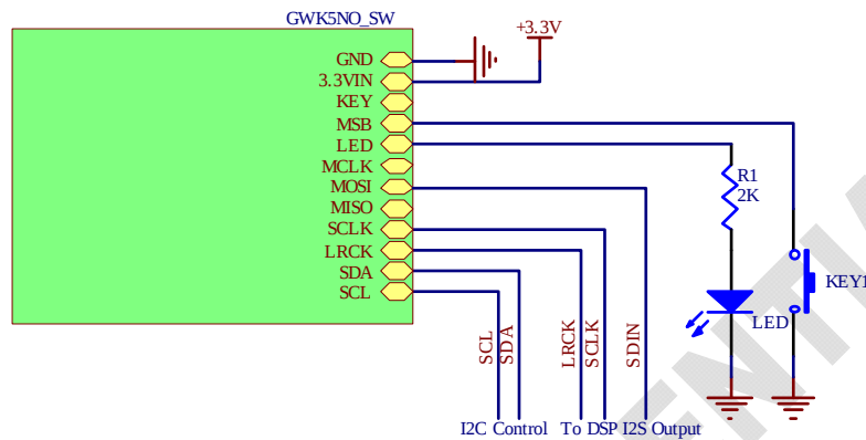
Figure [4]: GWK5NO_SW Interfacing with DSP (I2S Slave Input Mode)
