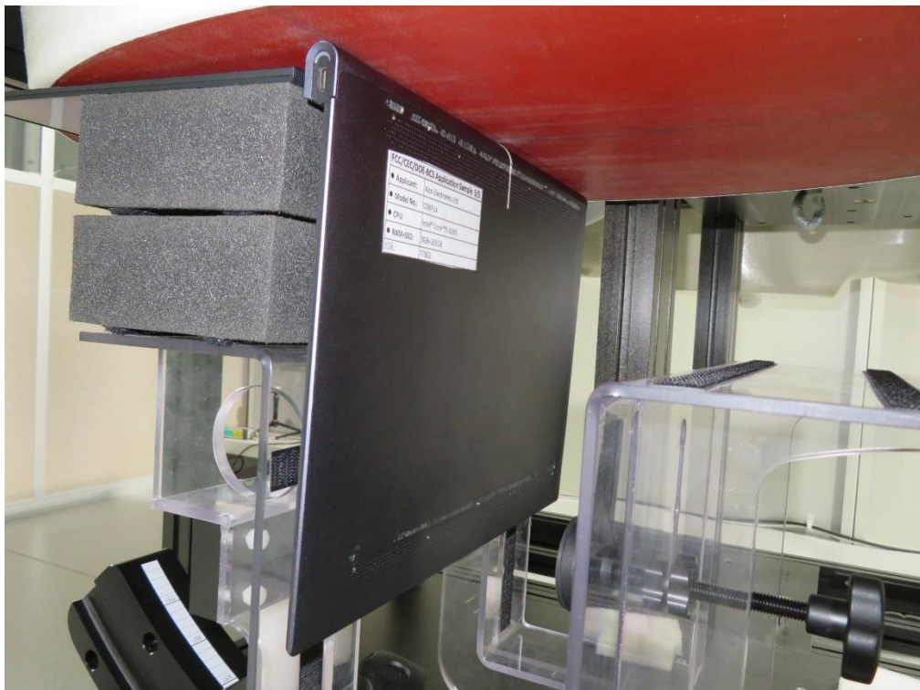
Description: SAR Test Setup Screen Side with 0mm gap
