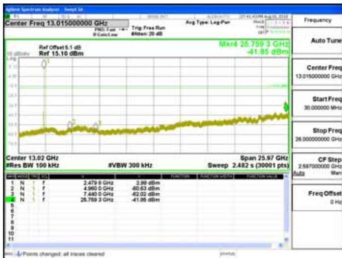
Spurious Emission_GFSK_1M_DH5_2480MHz
