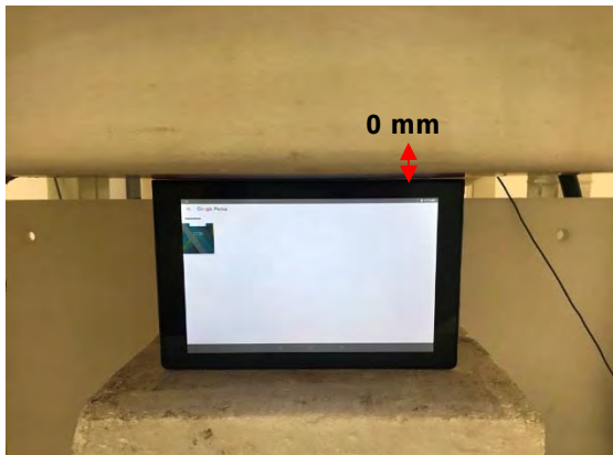
Fig.7 EUT Bottom side to flat phantom
