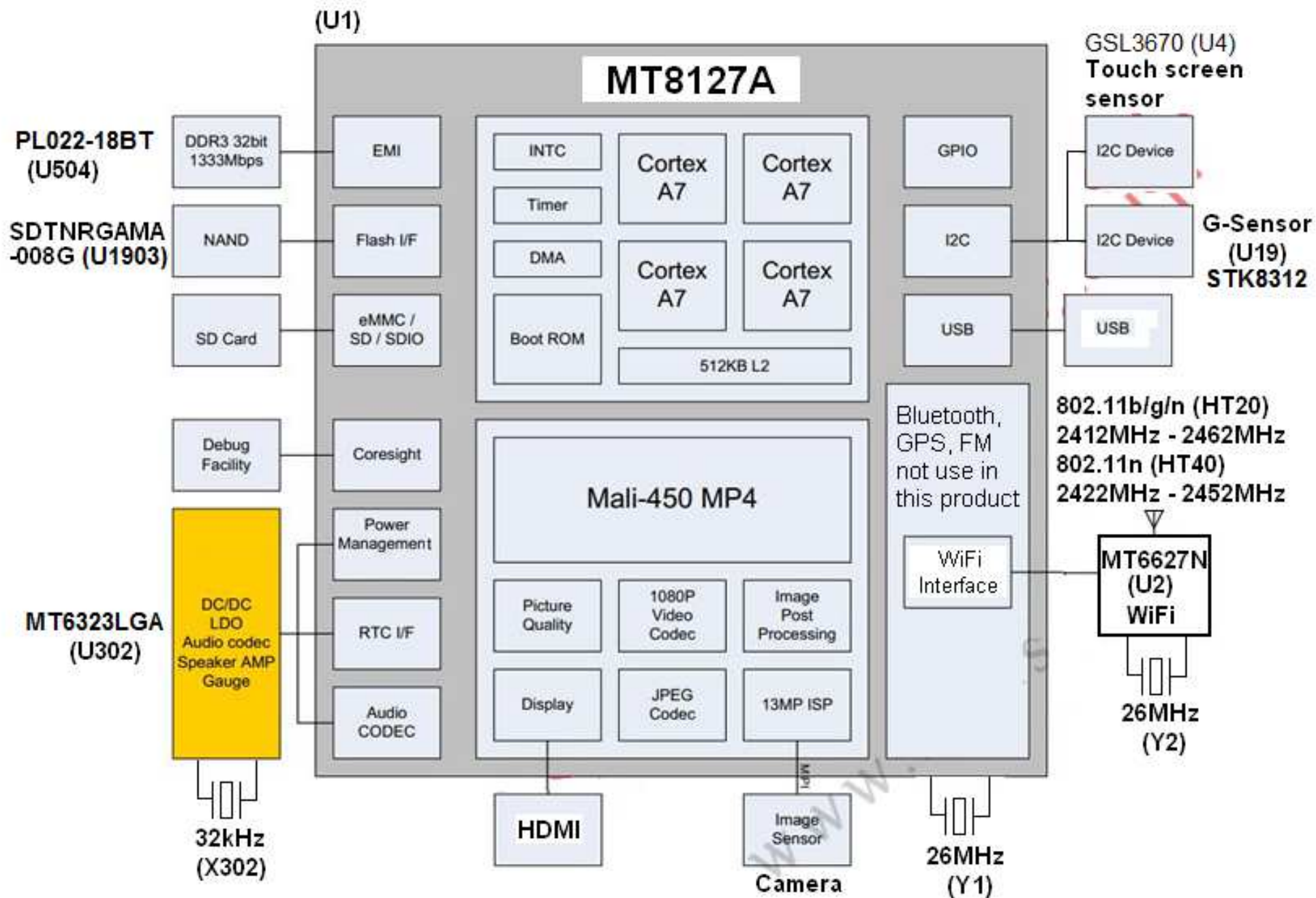
Block Diagram
