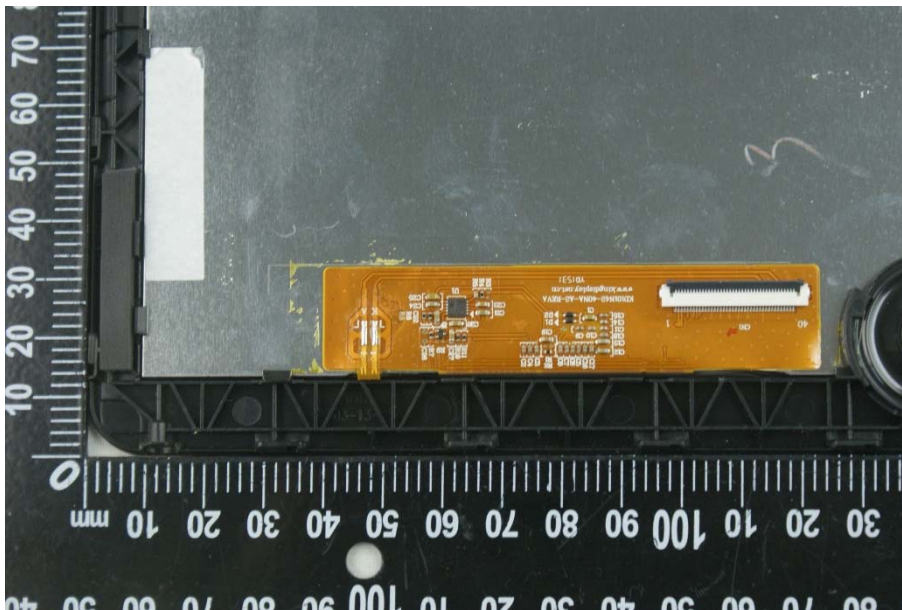
MAIN BOARD TOP VIEW 5
