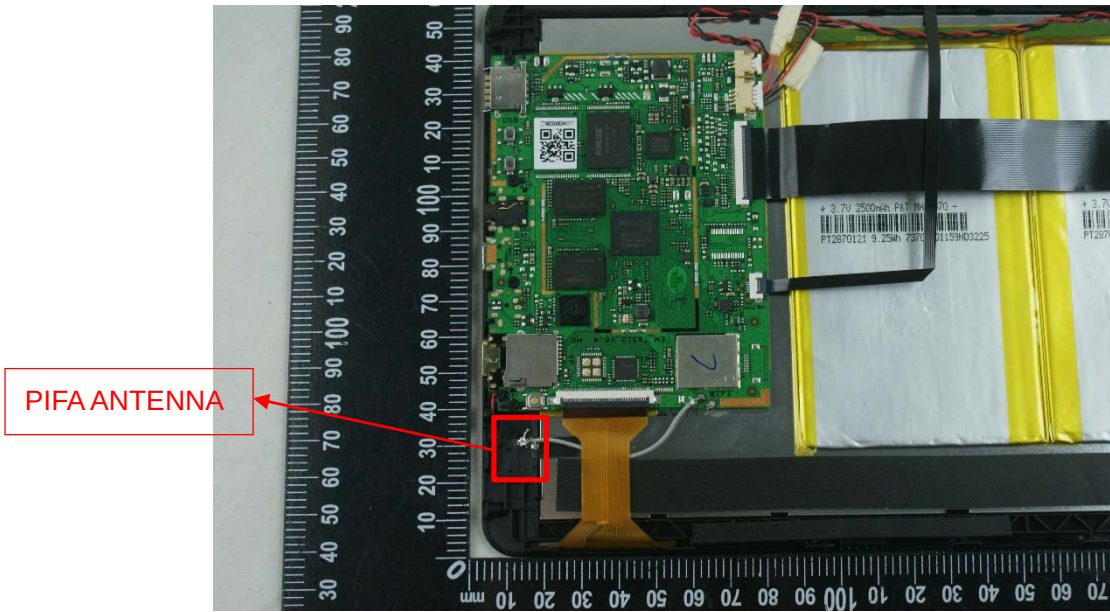
EUT UNCOVER VIEW 3
