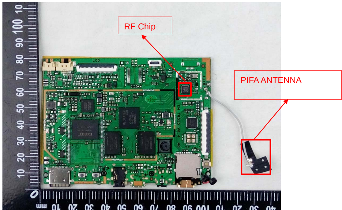
MAIN BOARD TOP VIEW 2
