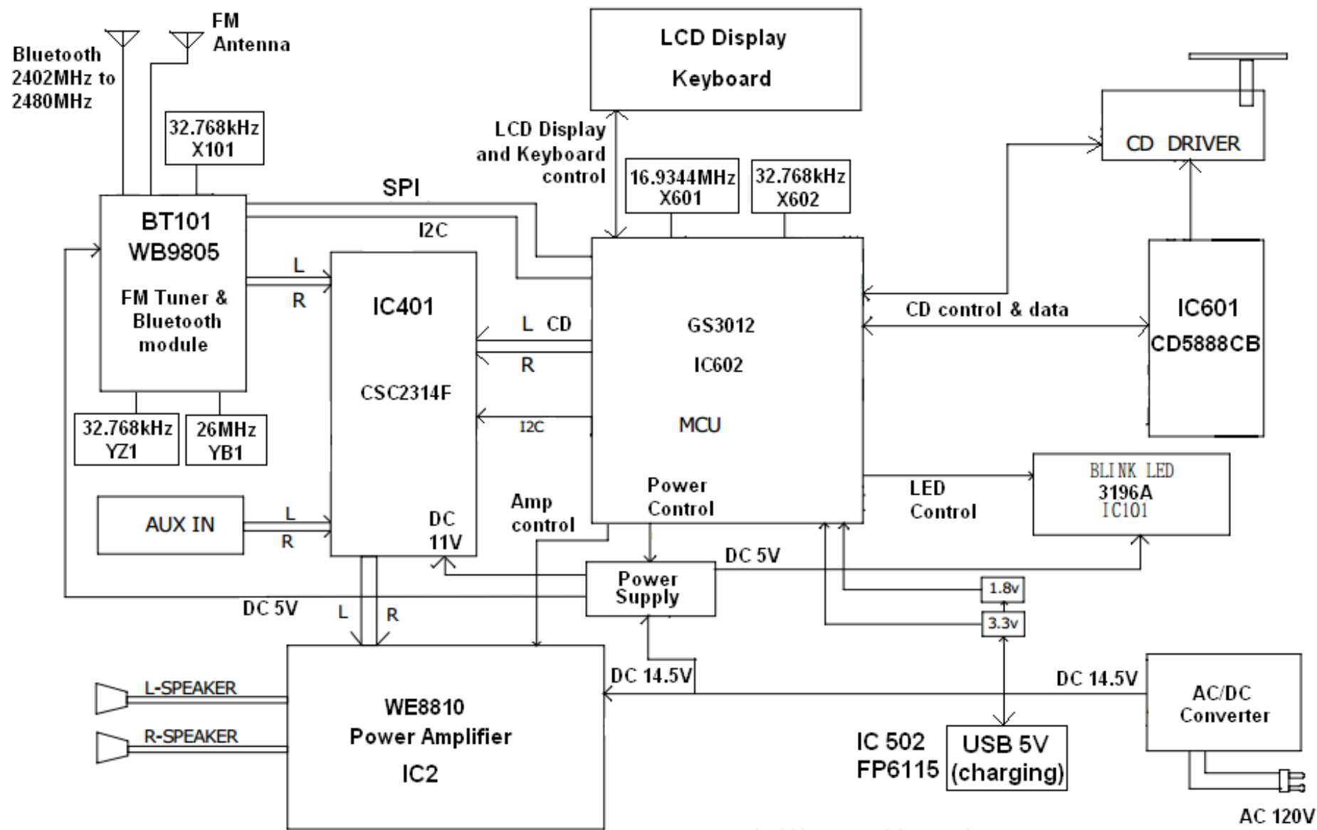
CD6697BL BLOCK DIAGRAM
