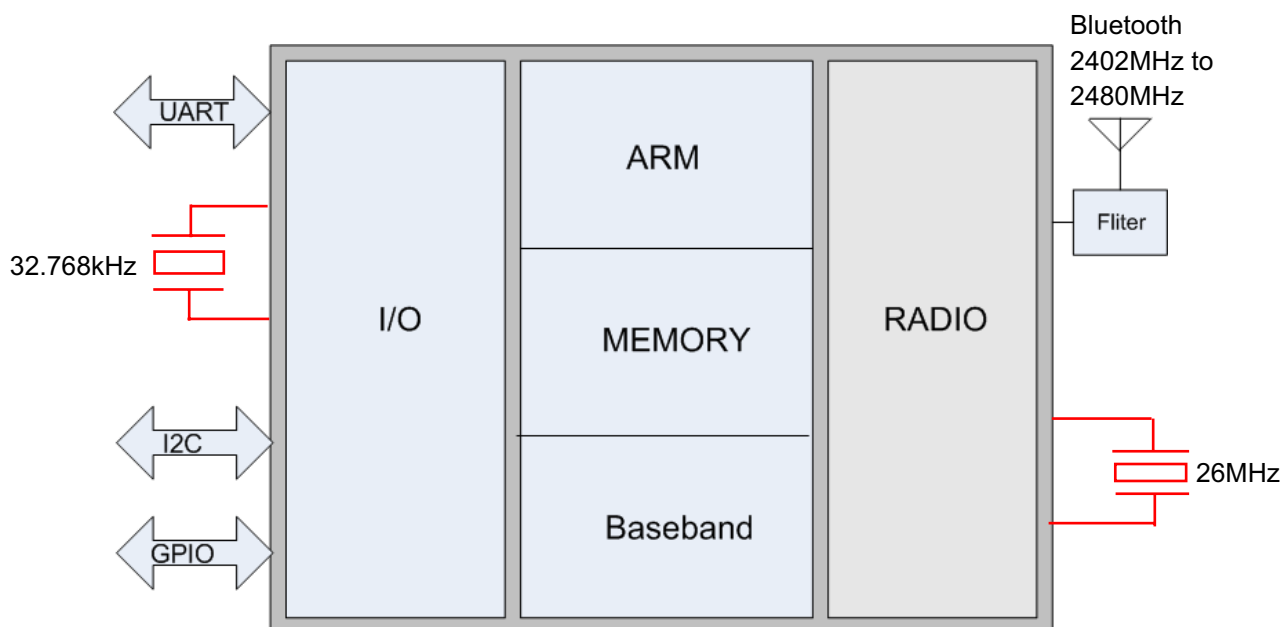
Figure3-1. RDA5876 Bluetooth Block Diagram
