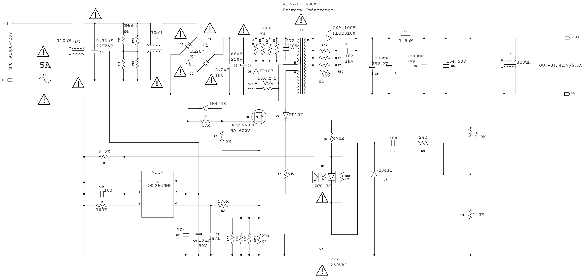
Power Supply
