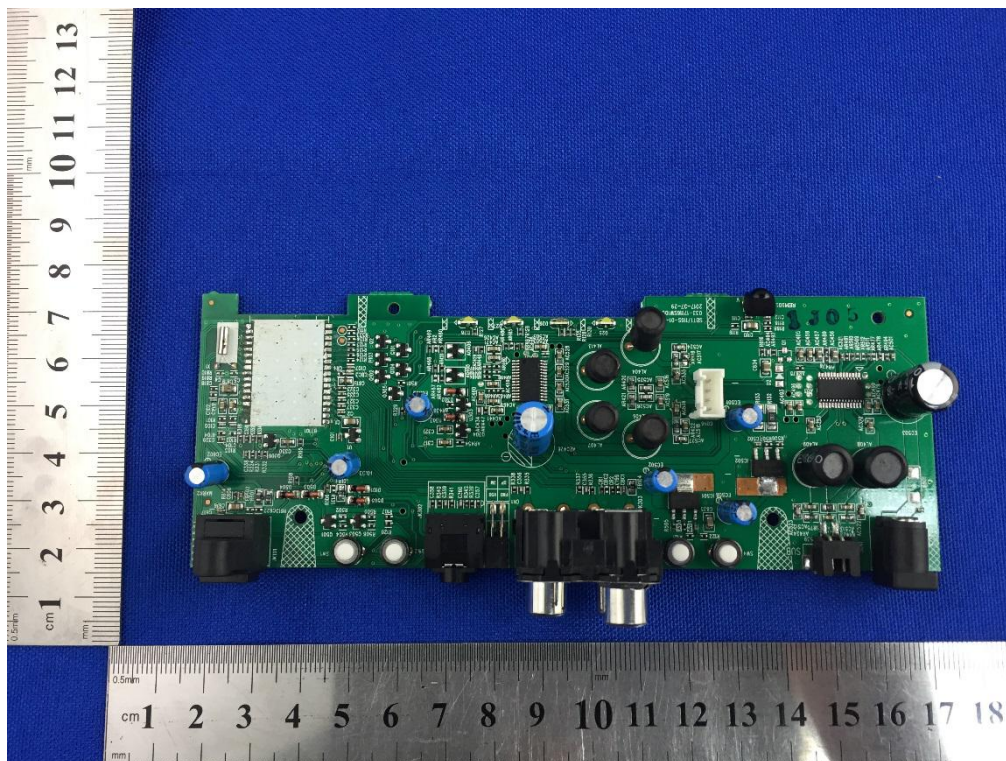
EUT 1 MAIN BOARD TOP VIEW 2
