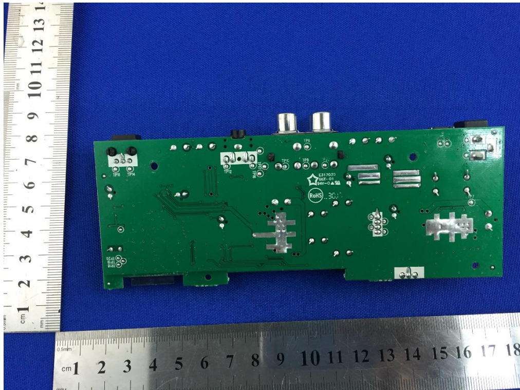
EUT 1 MAIN BOARD BACK VIEW 2
