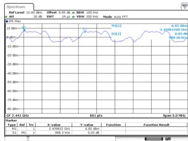
8-DPSK
