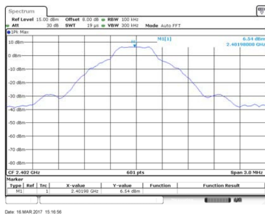
GFSK LOW CHANNEL, CARRIER LEVEL
