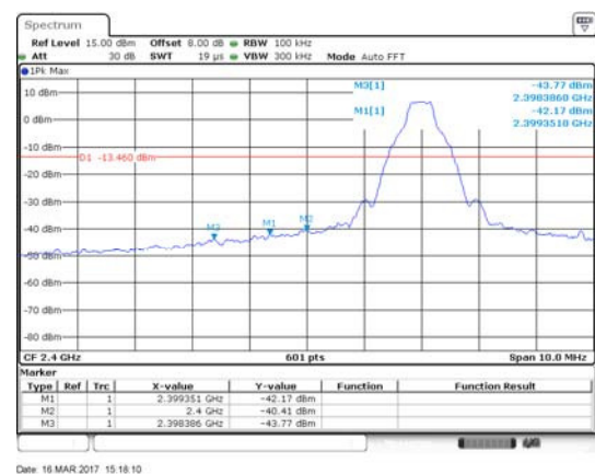
GFSK LOW CHANNEL, BAND EDGE
