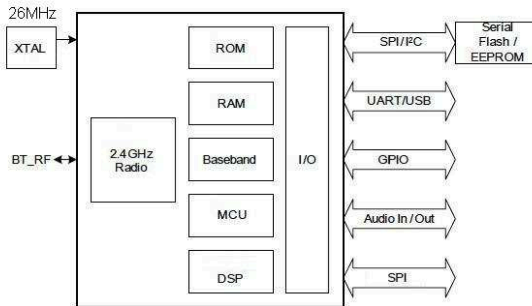
CW6682E Block Diagram
