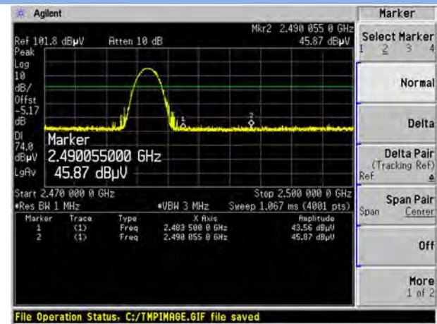
II/4-DQPSK HIGH CHANNEL , PEAK
