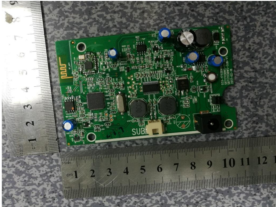
MAIN BOARD TOP VIEW 1 (Wireless Subwoofer)
