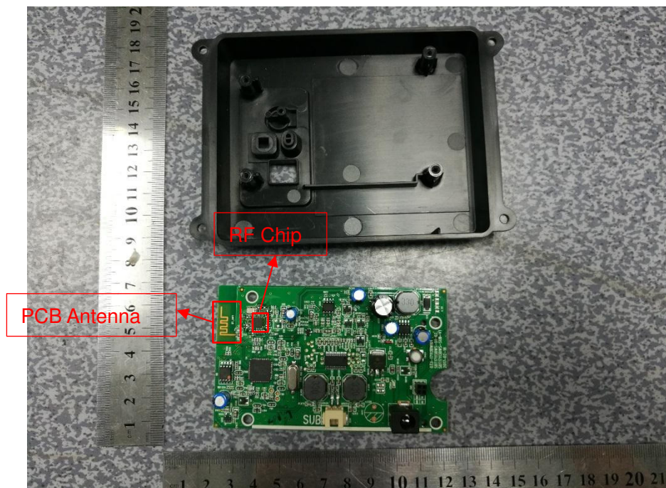
EUT UNCOVER VIEW 2 (Wireless Subwoofer)
