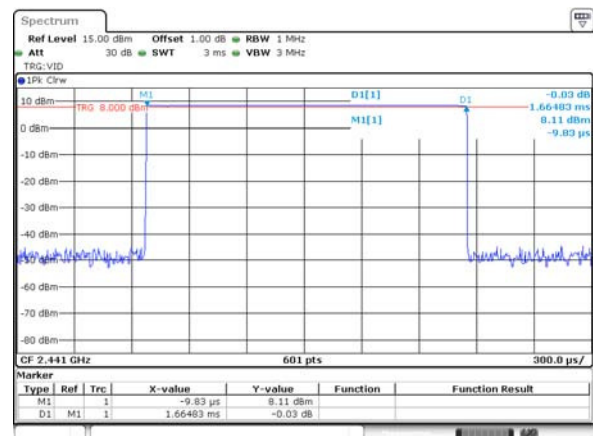
GFSK DH3
