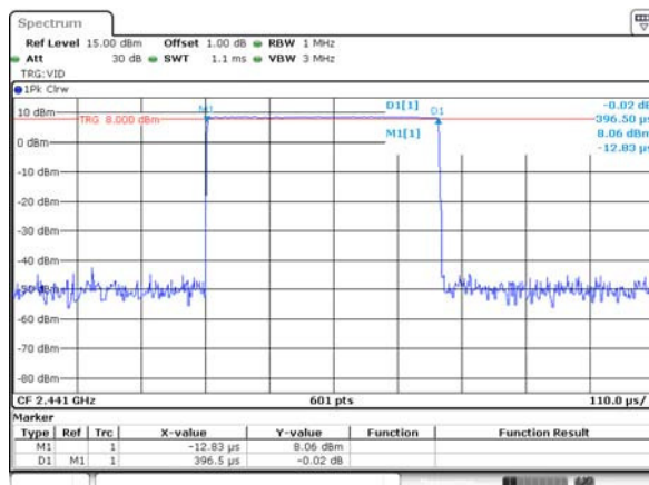
GFSK DH1
