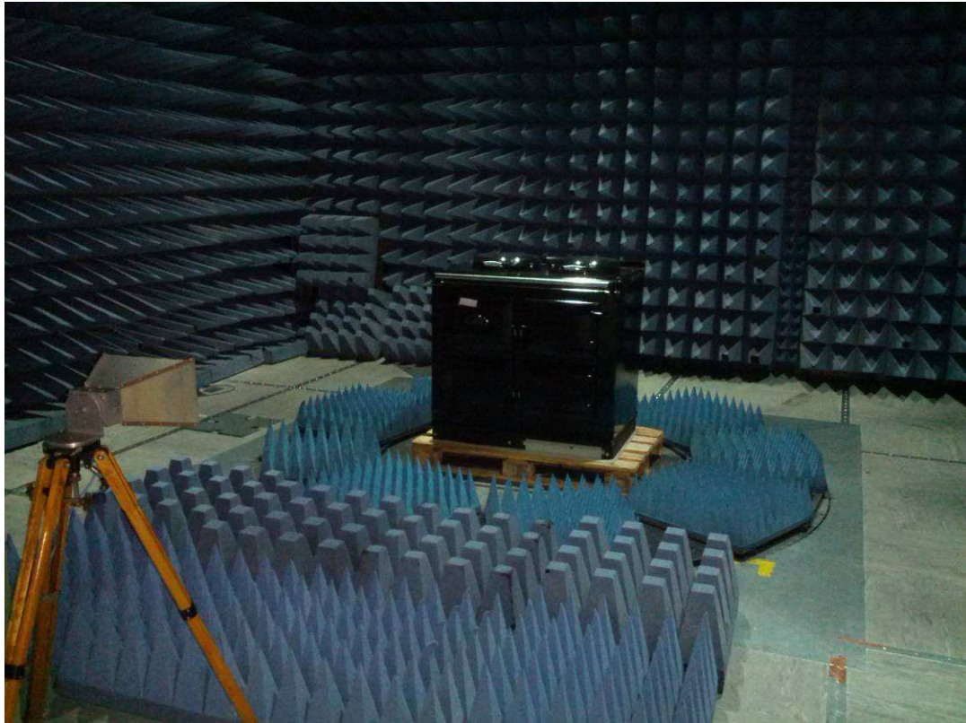
Radiated Power and Spurious Emissions 1- 10GHz
