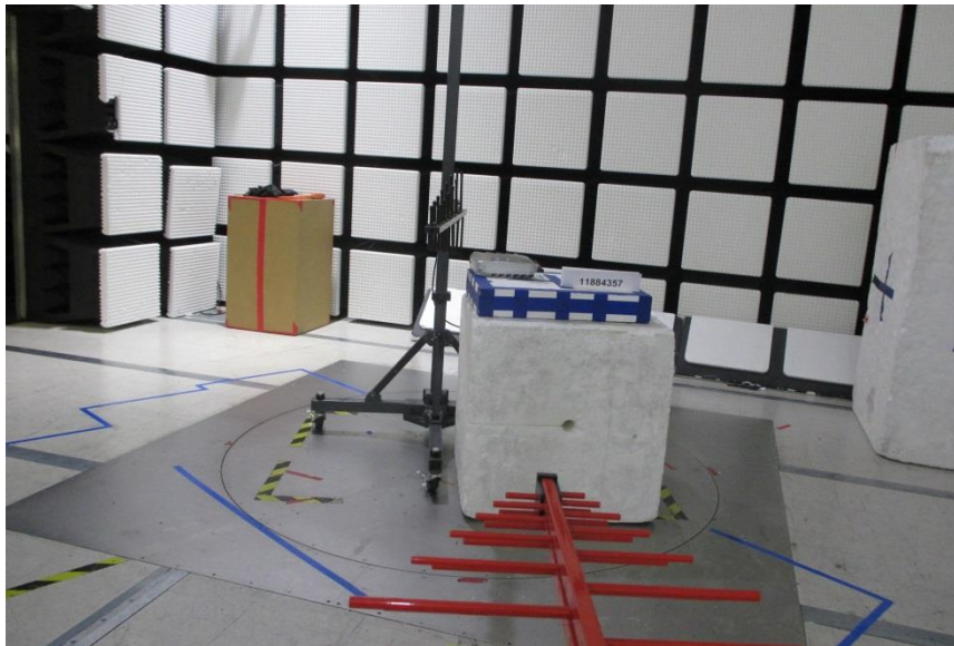
RADIATED BACK UHF LOG PERIODIC ANTENNA
