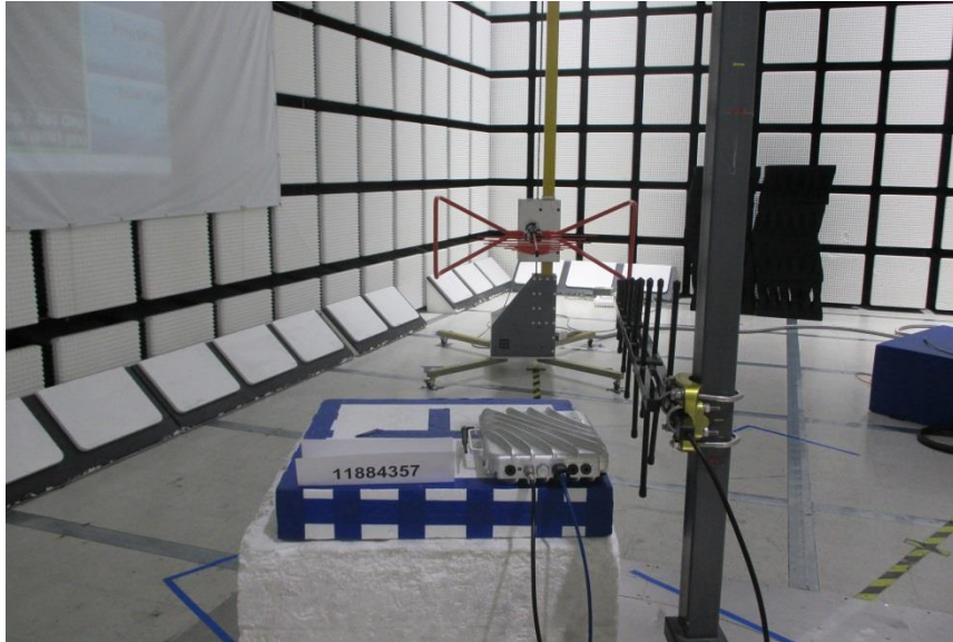
RADIATED FRONT UHF LOG PERIODIC ANTENNA
