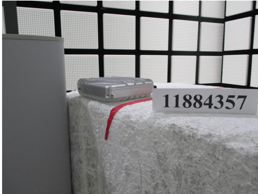
RADIATED FRONT UHF PANEL ANTENNA
