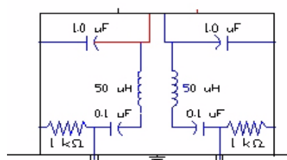
Figure 4. LISN Schematic Diagram
