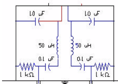
Figure 5. LISN Schematic Diagram
