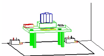
Figure 2. Line Conducted Emission Test Set-Up
