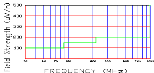
Figure 10. Limits at 3 meters
