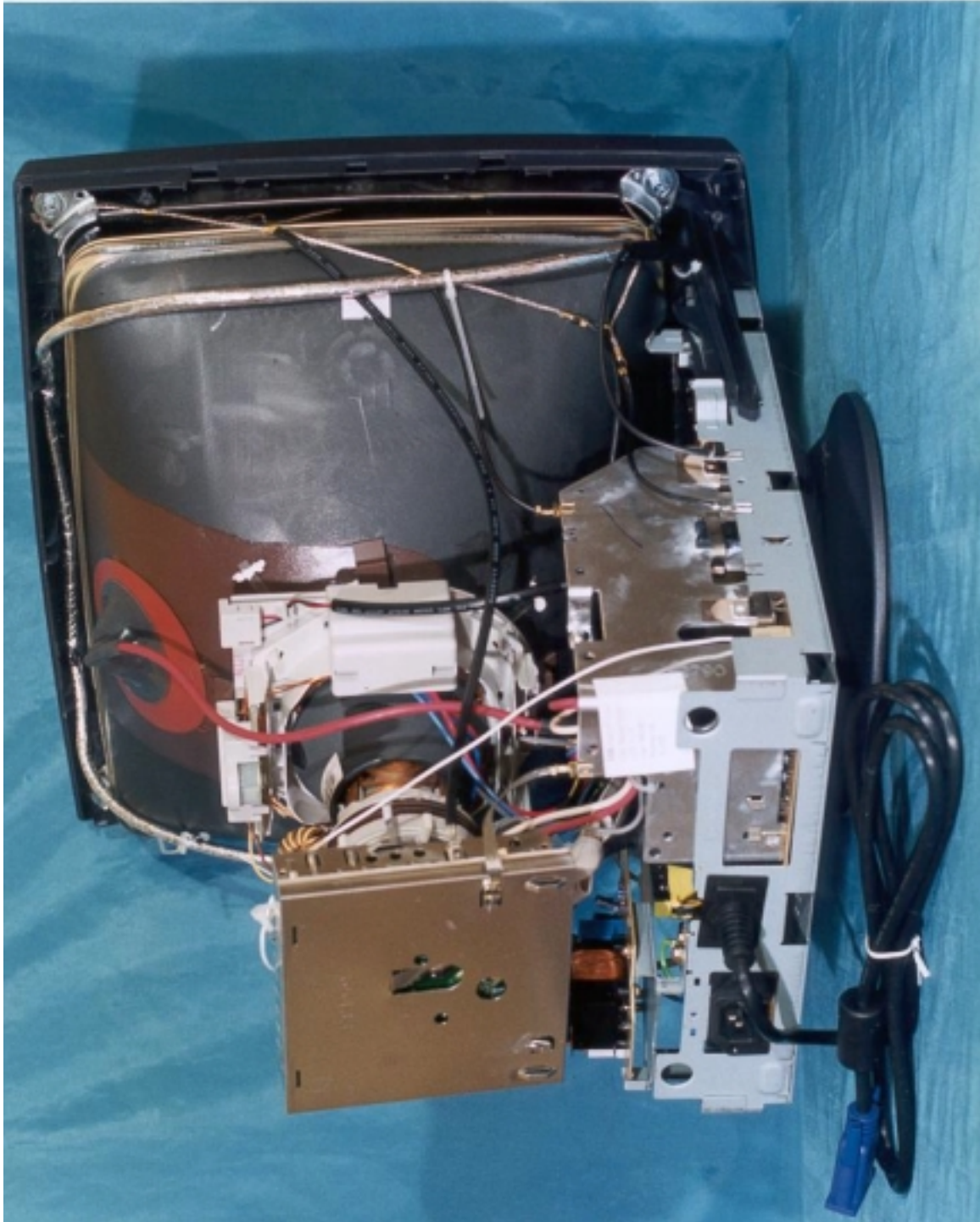
Side View w/o Back Cover
