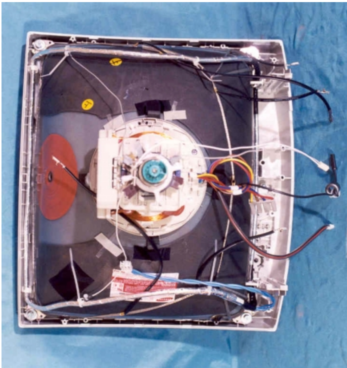
CRT Assembly
