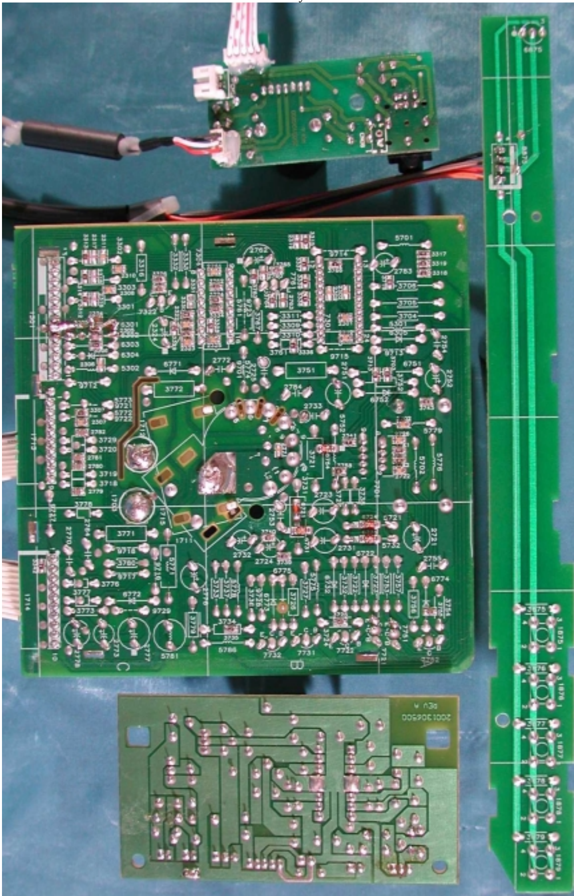
PCB Layout
