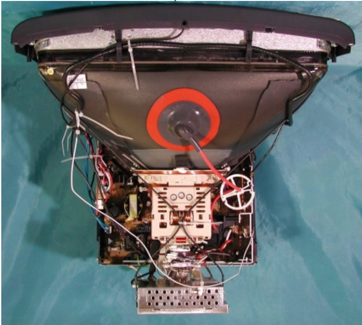
Top View
