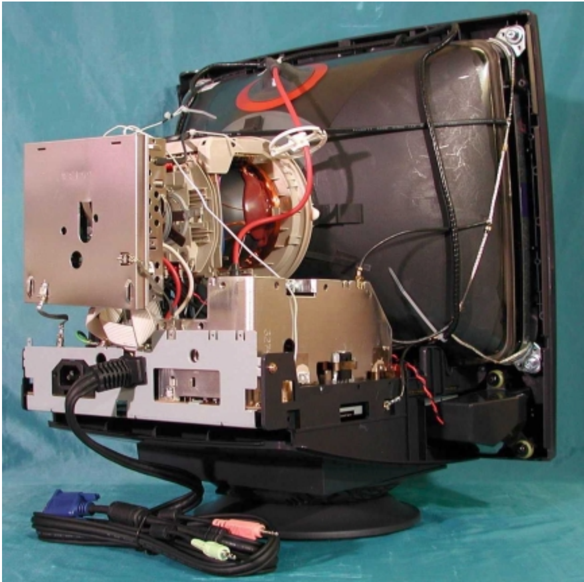
Side View
