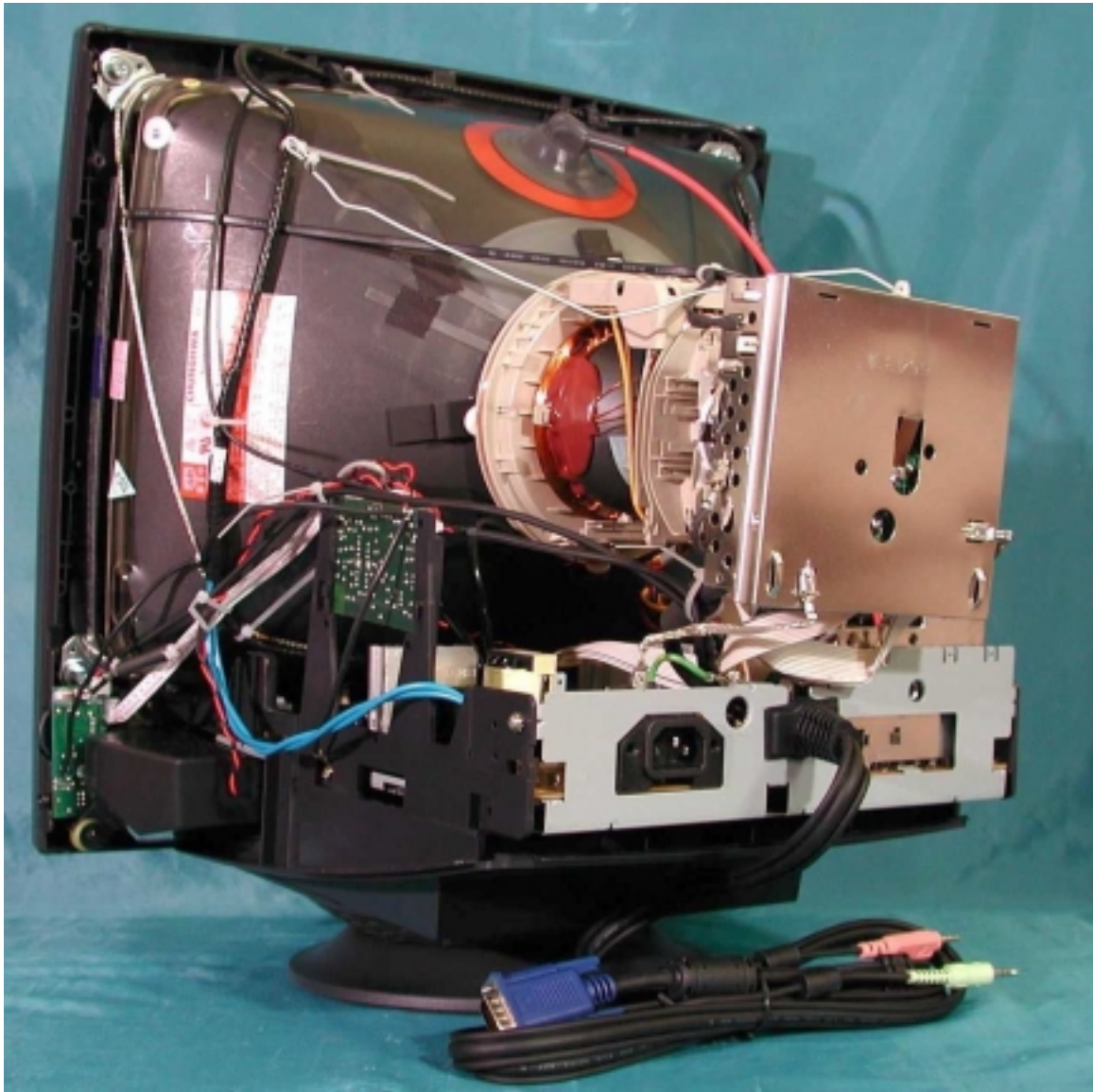
Side View
