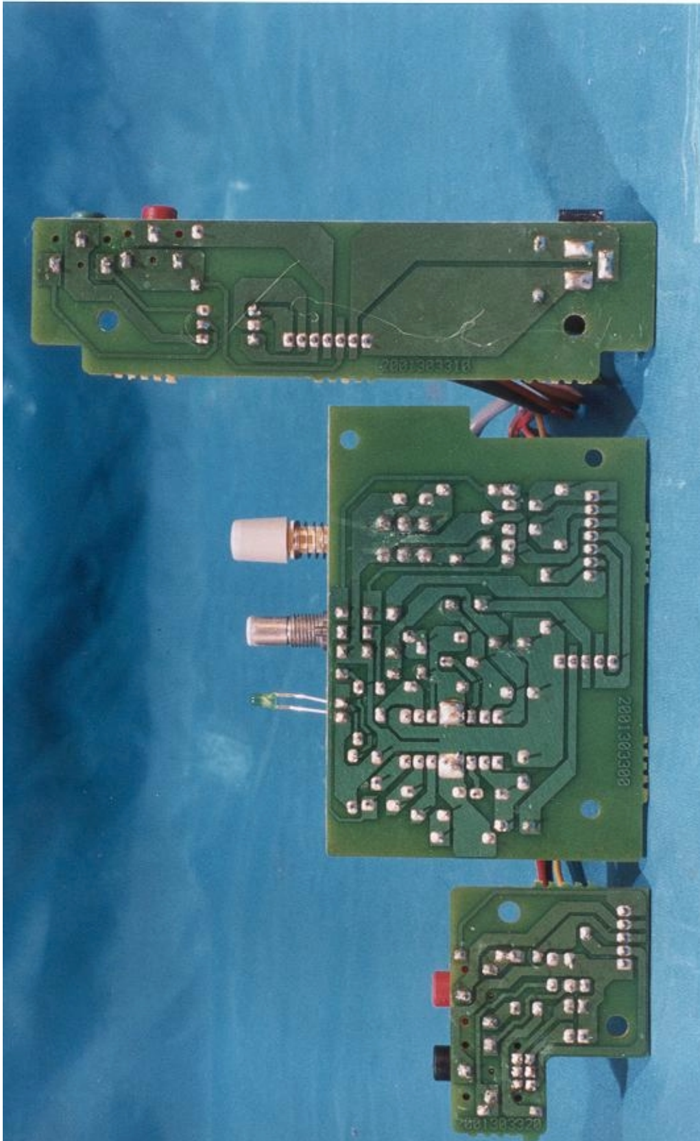
PCB Layout
