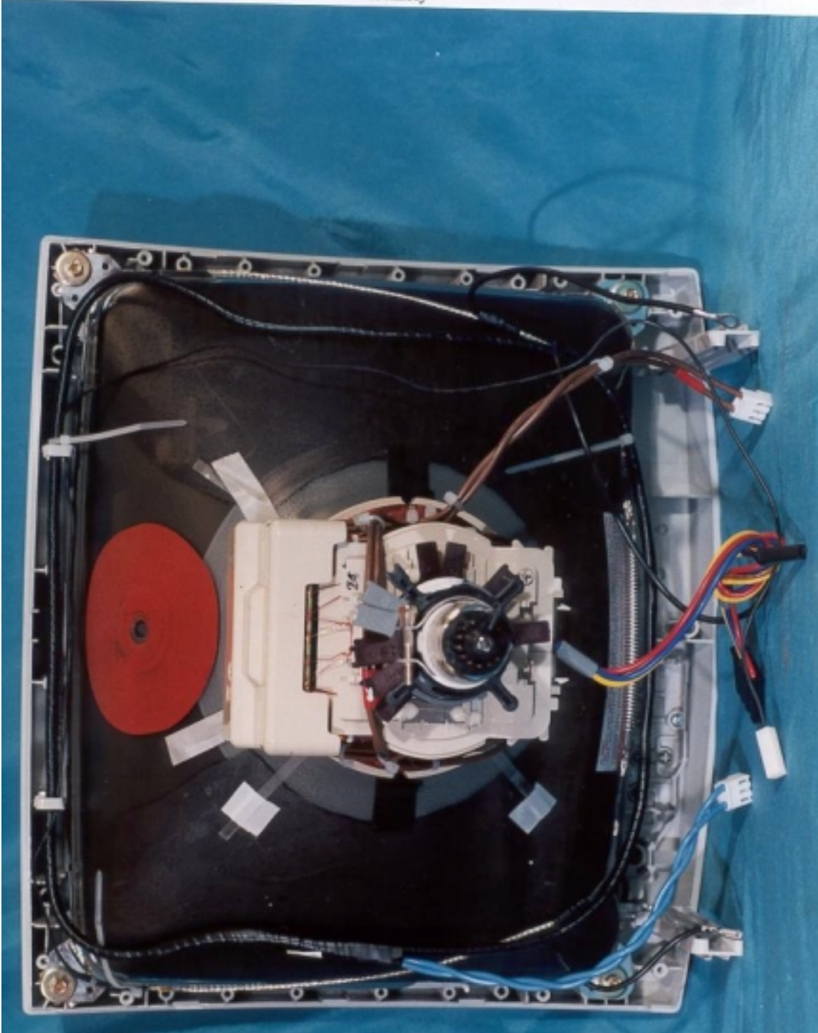
CRT Assembly
