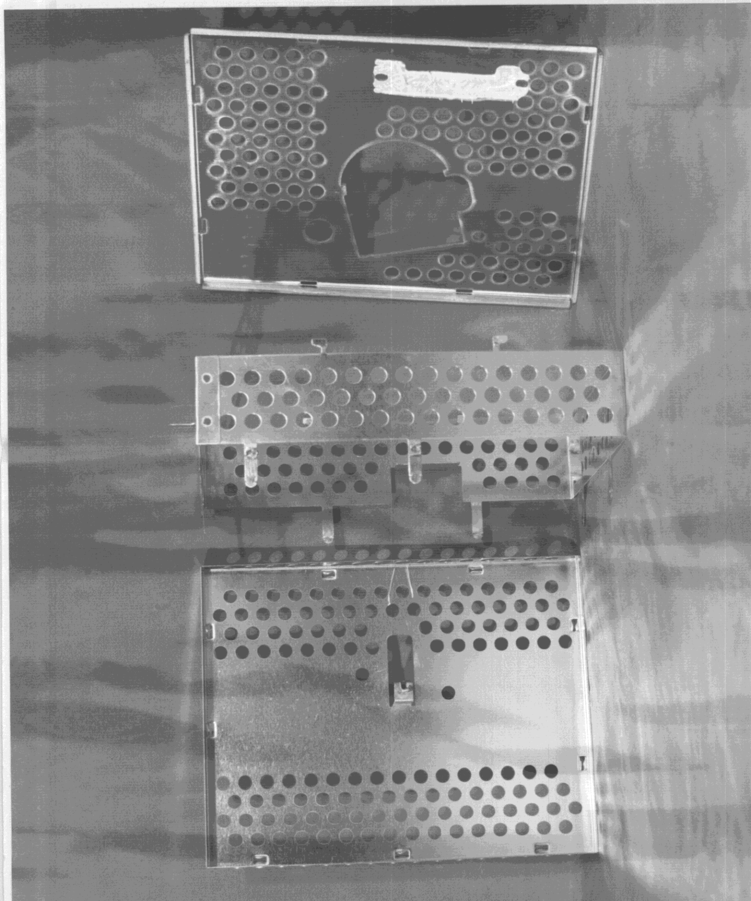
Shielding Cover
