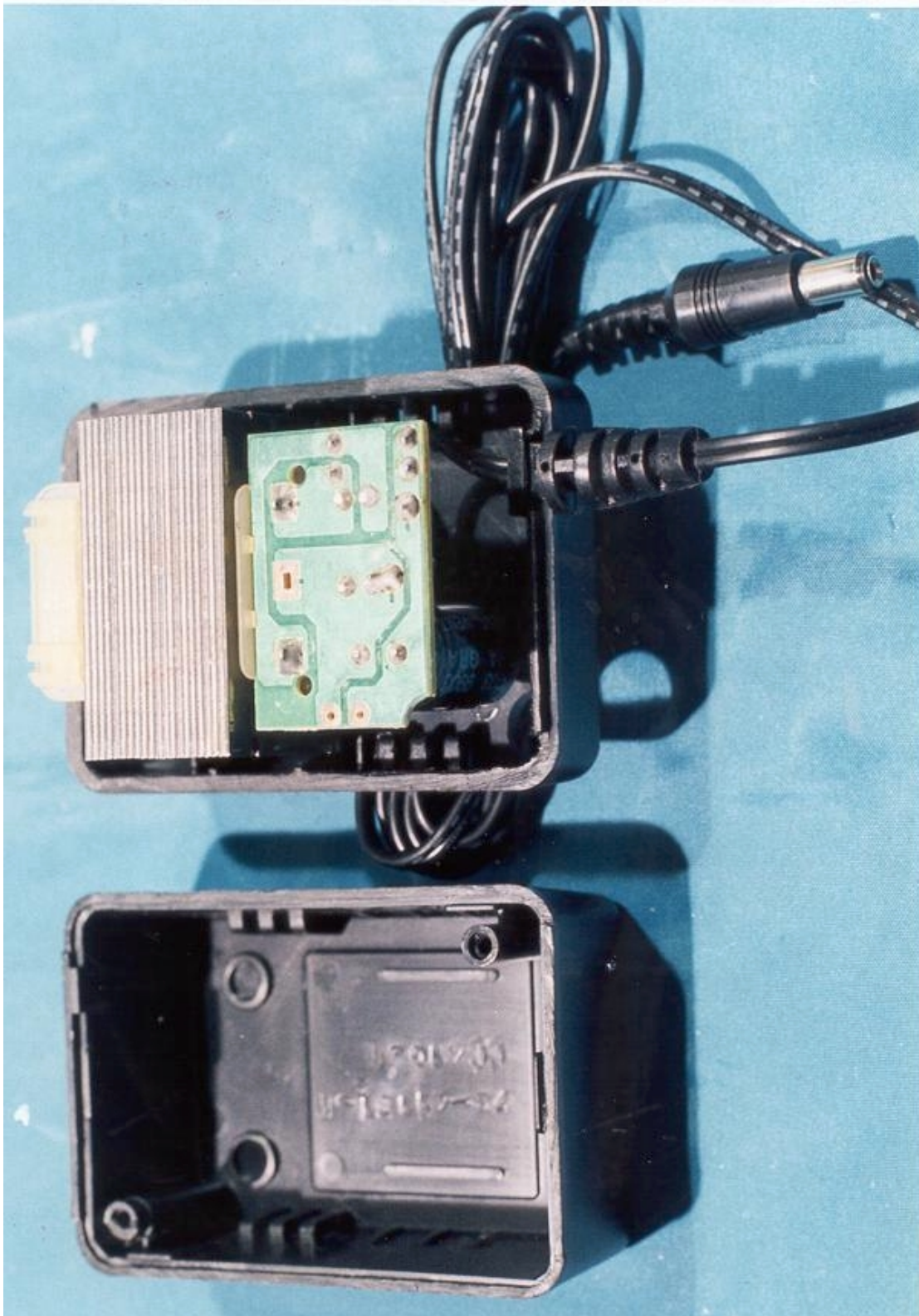
AC Adapter - Layout
