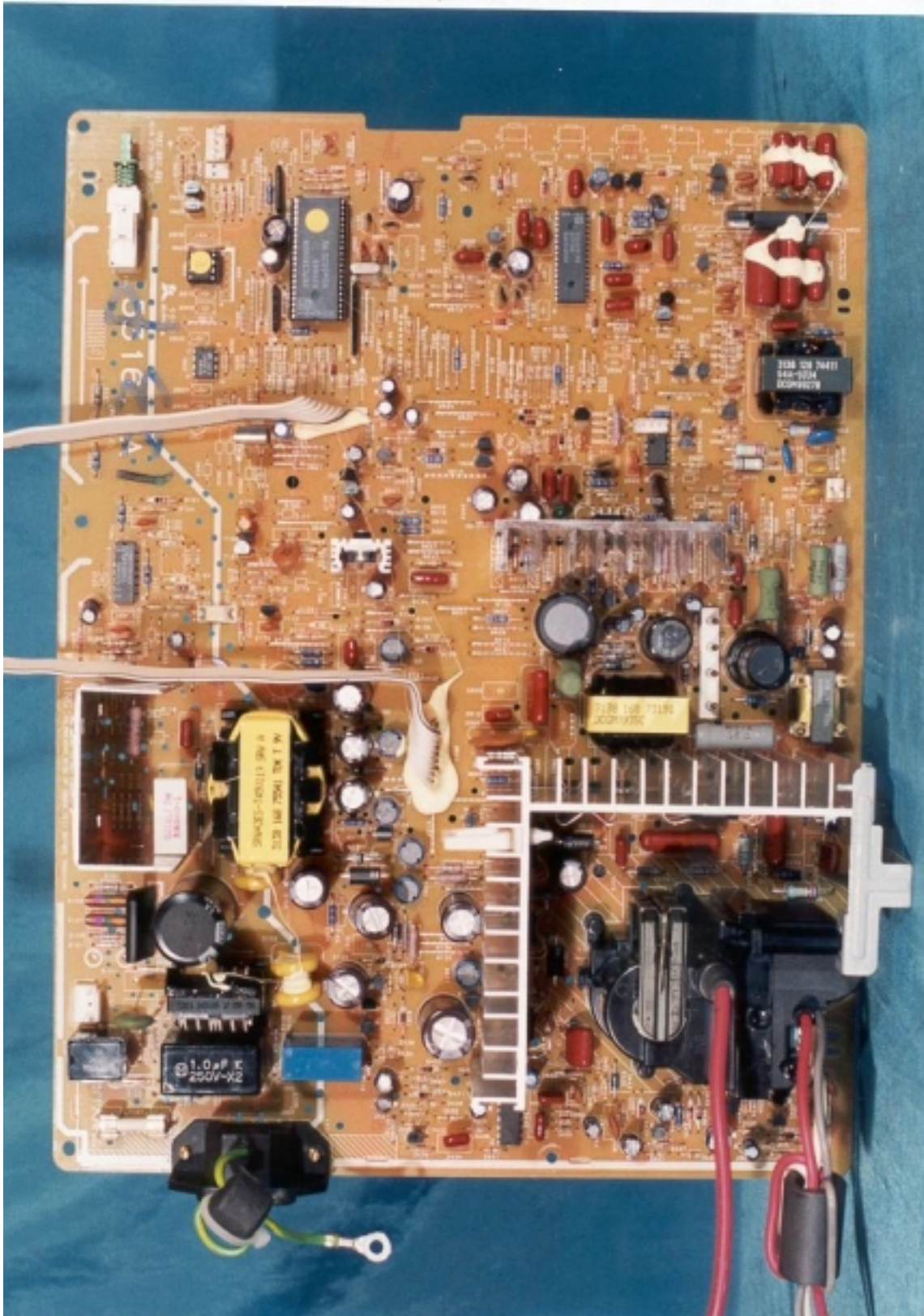
PCB Layout
