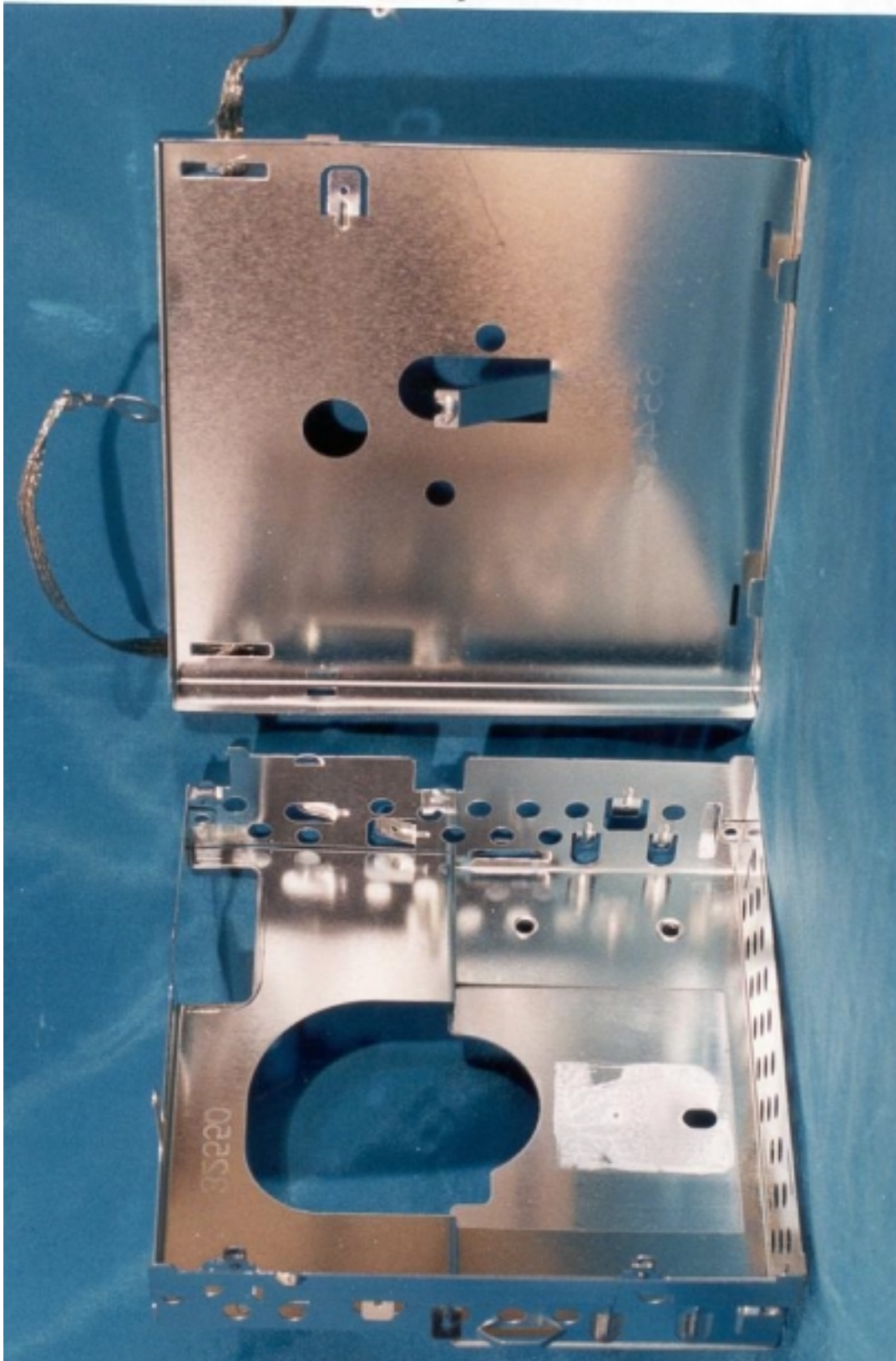
Shielding Cover
