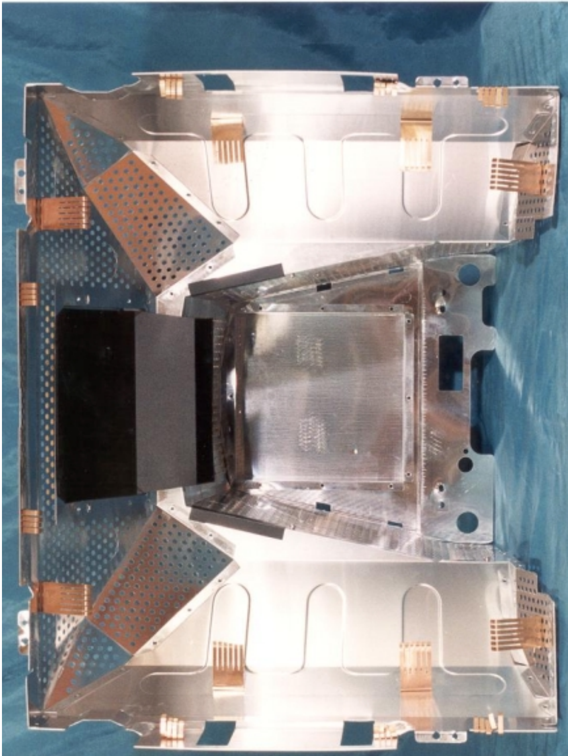
Shielding Cover
