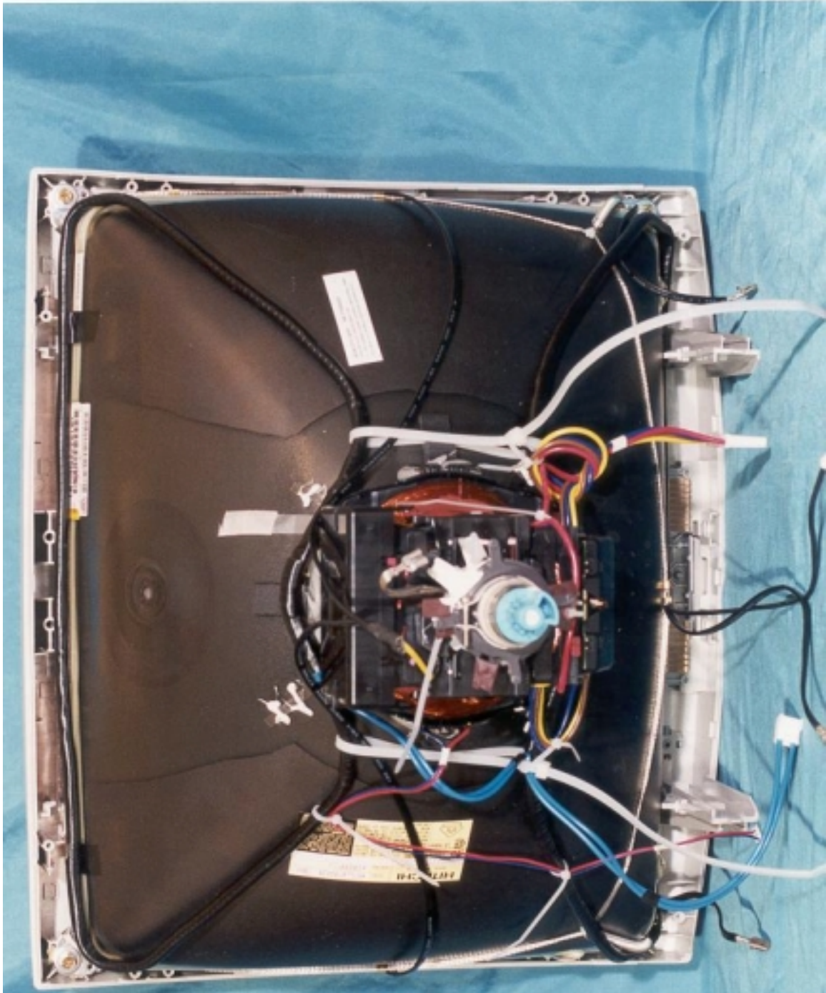
CRT Assembly
