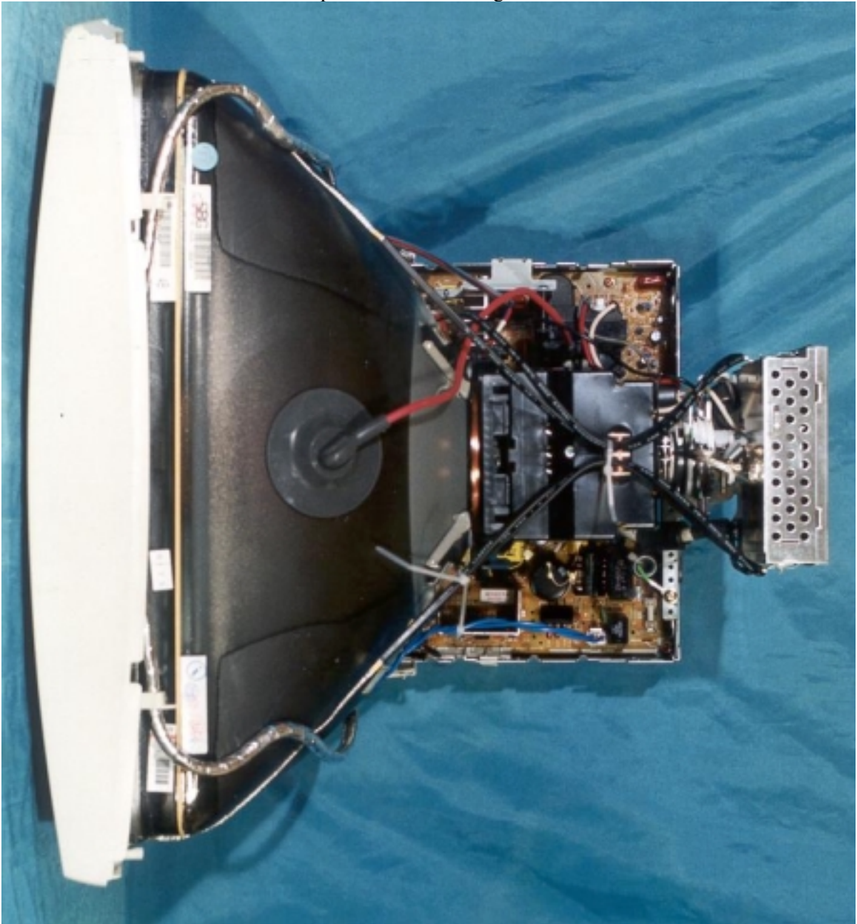
Top View w/o Shielding Cover
