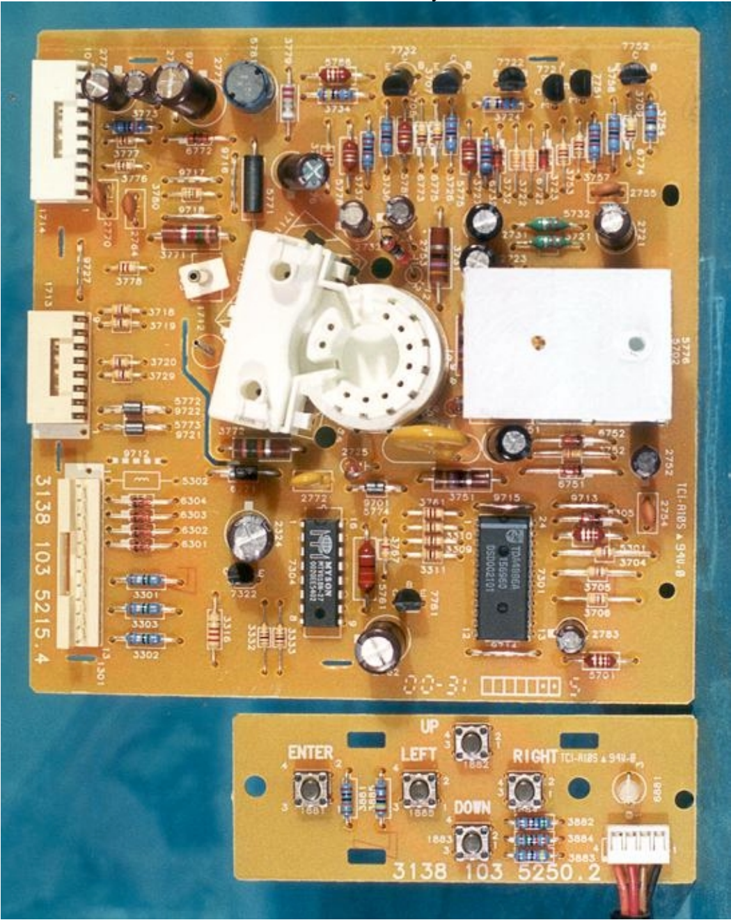
PCB Layout
