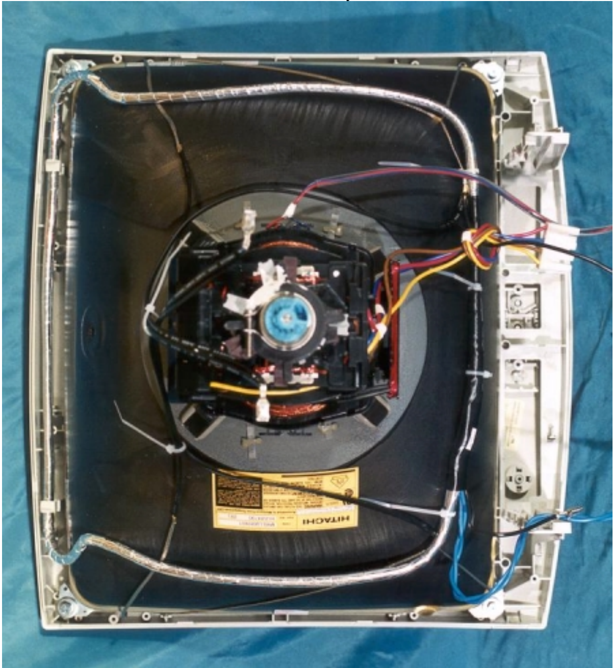
CRT Assembly
