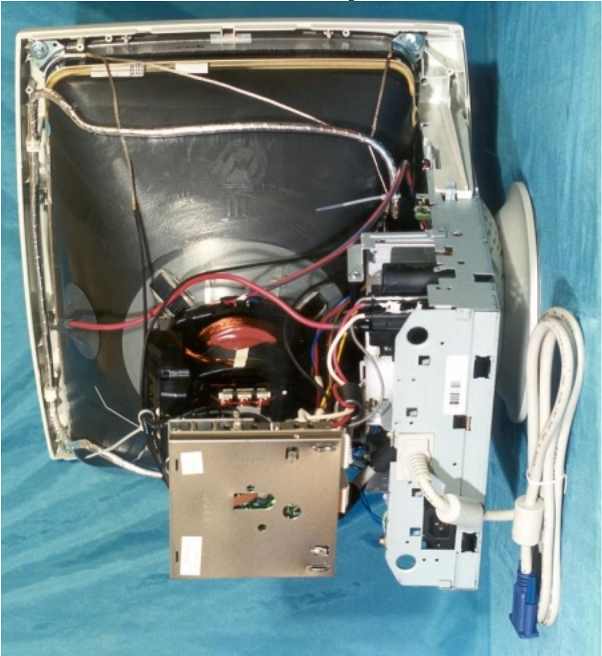
Side View w/o Shielding Cover
