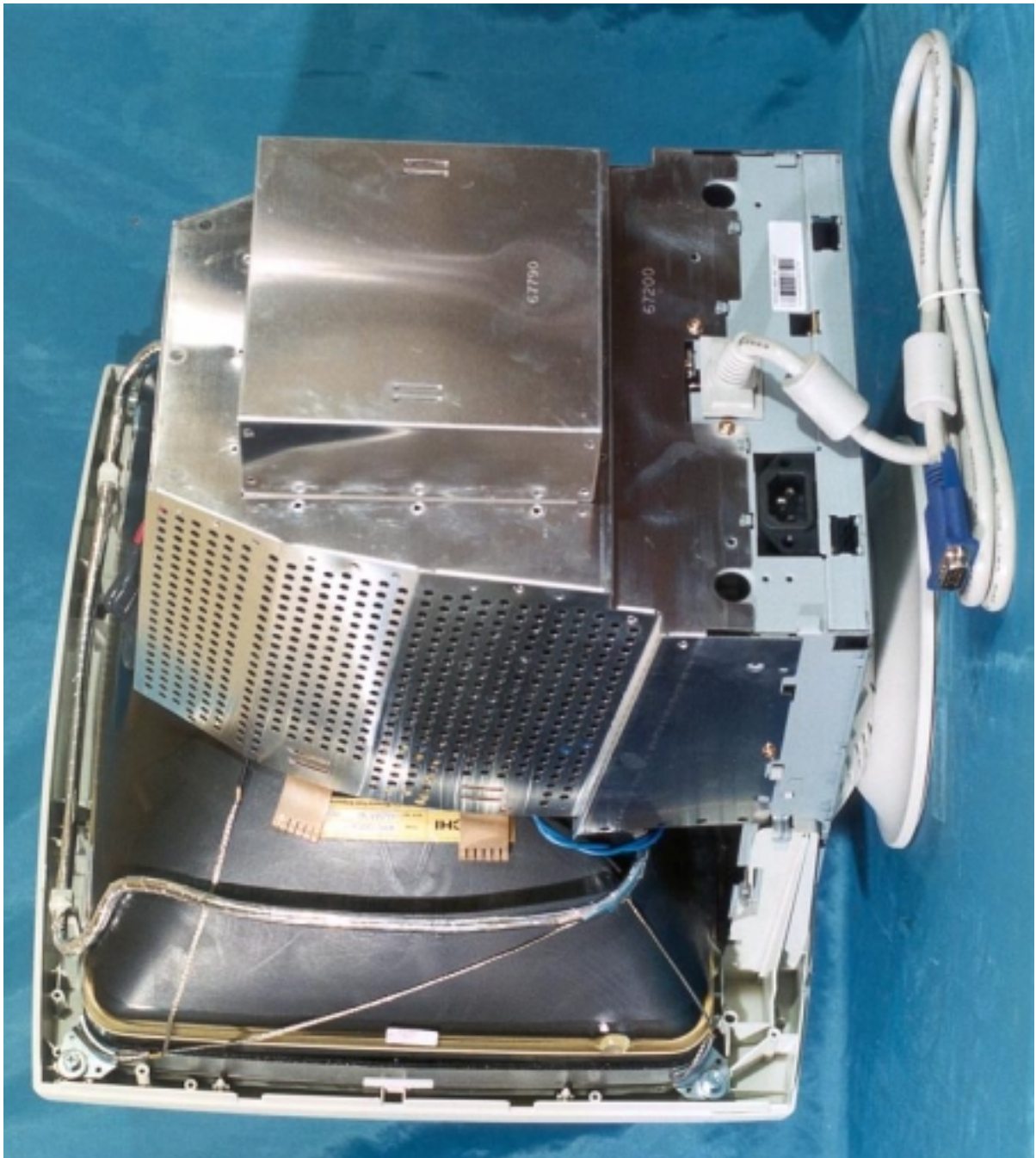
Side View w/o Back Cover
