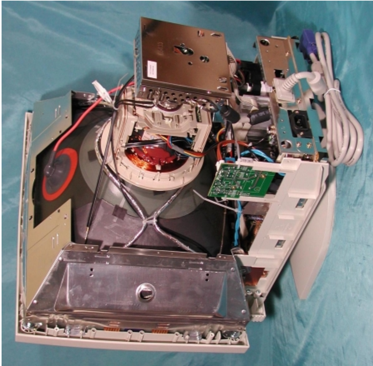
Side View Without Shielding Cover
