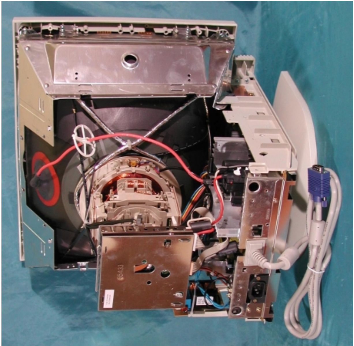
Side View Without Shielding Cover
